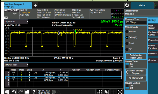
802.11ax-HE20 (T=777.7us)
