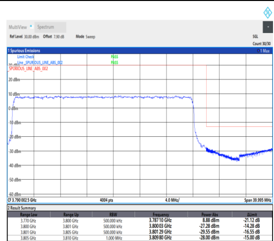
1-N78-3700-3800--30-30-H-3-DFT-PI2BPSK-Outer_Full-75@0-Ant1-1--PASS-see graph
