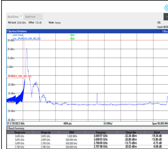
1-N78-3700-3800--30-80-L-4-CP-QPSK-Edge_1RB_Left-1@0-Ant1-1--PASS-see graph
