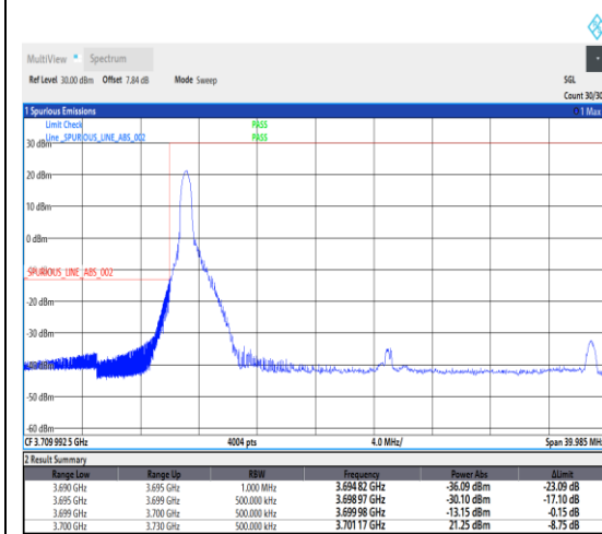
1-N78-3700-3800--30-30-L-4-CP-QPSK-Edge_1RB_Left-1@0-Ant1-1--PASS-see graph
