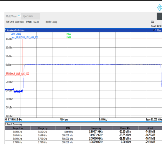
1-N78-3700-3800--30-80-L-6-CP-QPSK-Outer_Full-217@0-Ant1-1--PASS-see graph
