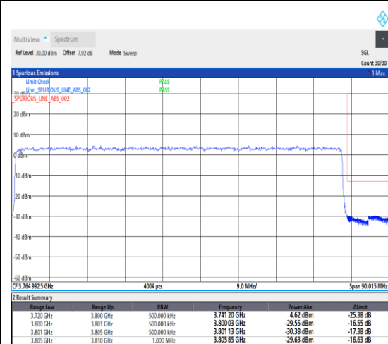
1-N78-3700-3800--30-80-H-3-DFT-PI2BPSK-Outer_Full-216@0-Ant1-1--PASS-see graph
