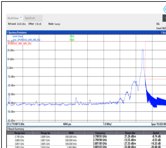
1-N78-3700-3800--30-60-H-2-DFT-PI2BPSK-Edge_1RB_Right-1@161-Ant1-1--PASS-see graph
