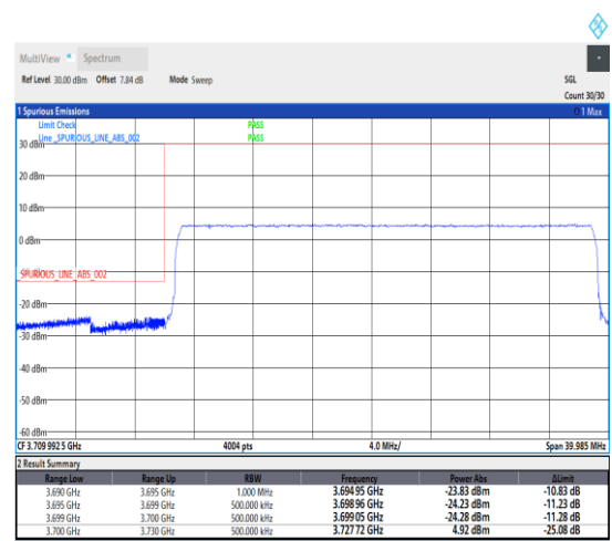
1-N78-3700-3800--30-30-L-6-CP-QPSK-Outer_Full-78@0-Ant1-1--PASS-see graph
