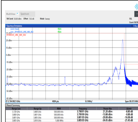
1-N78-3700-3800--30-80-H-2-DFT-PI2BPSK-Edge_1RB_Right-1@216-Ant1-1--PASS-see graph
