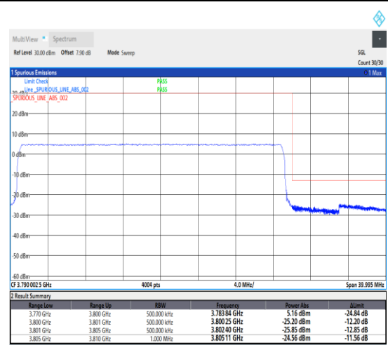
1-N78-3700-3800--30-30-H-3-DFT-PI2BPSK-Outer_Full-75@0-Ant1-1--PASS-see graph
