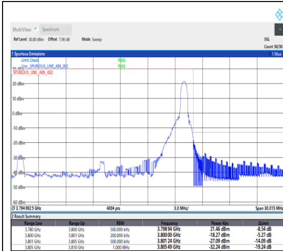
1-N78-3700-3800--30-20-H-2-DFT-PI2BPSK-Edge_1RB_Right-1@50-Ant1-1--PASS-see graph
