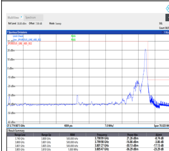
1-N78-3700-3800--30-60-H-5-CP-QPSK-Edge_1RB_Right-1@161-Ant1-1--PASS-see graph
