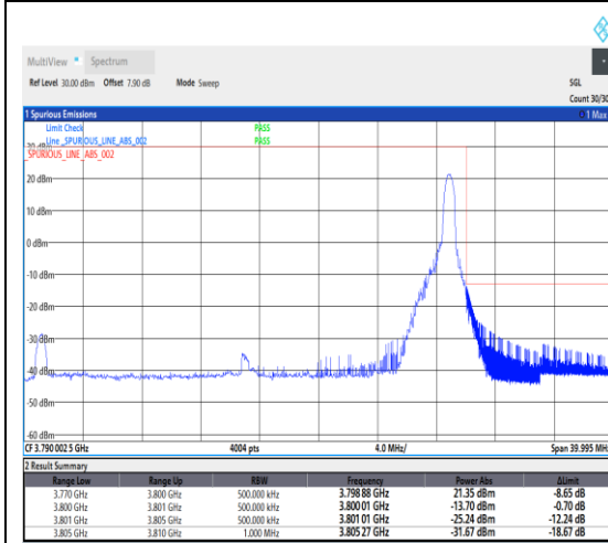
1-N78-3700-3800--30-30-H-2-DFT-PI2BPSK-Edge_1RB_Right-1@77-Ant1-1--PASS-see graph
