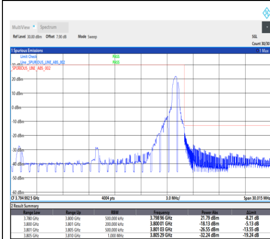
1-N78-3700-3800--30-20-H-5-CP-QPSK-Edge_1RB_Right-1@50-Ant1-1--PASS-see graph
