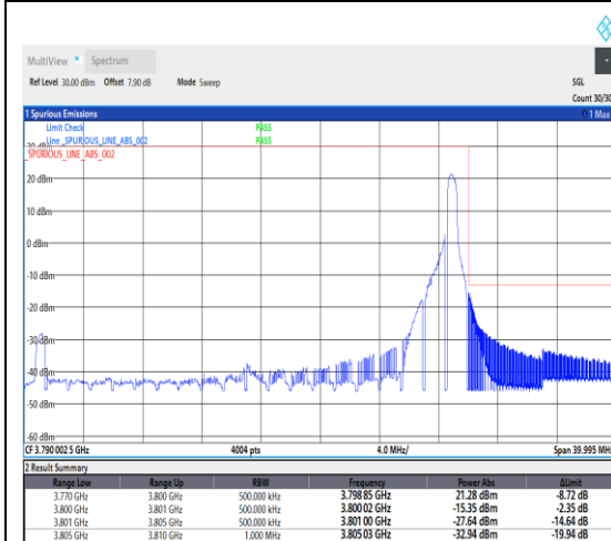
1-N78-3700-3800--30-30-H-2-DFT-PI2BPSK-Edge_1RB_Right-1@77-Ant1-1--PASS-see graph
