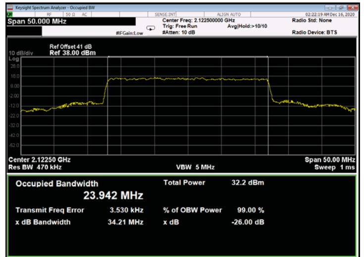
Figure 768: QPSK 25MHz B.W.; 2122.5MHz, 15kHz - Output
