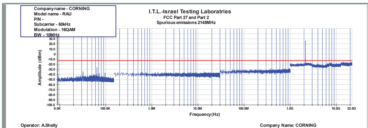
Figure 814: Spurious Emissions at Antenna Terminal 16QAM 10MHz B.W.; 2145.0MHz, 60kHz
