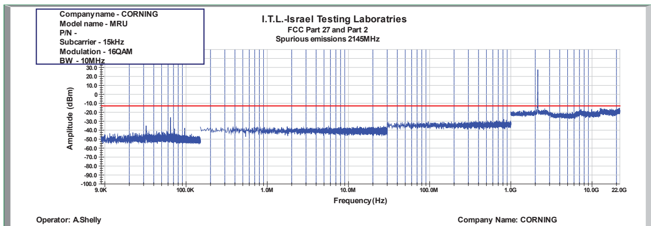
Figure 808: Spurious Emissions at Antenna Terminal 16QAM 10MHz B.W.; 2145.0MHz, 15kHz
