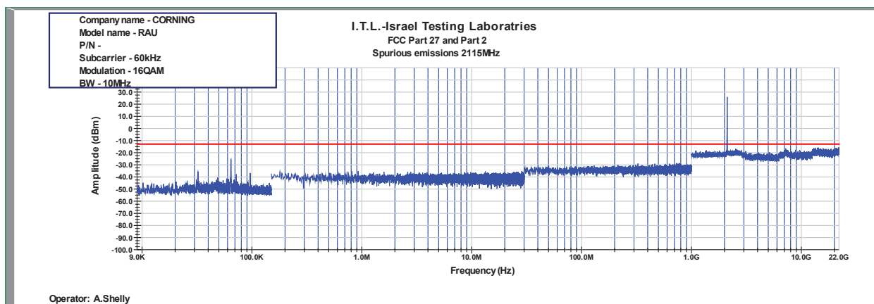
Figure 813: Spurious Emissions at Antenna Terminal 16QAM 10MHz B.W.; 2115.0MHz, 60kHz
