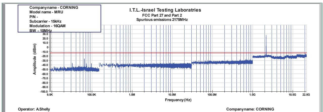
Figure 809: Spurious Emissions at Antenna Terminal 16QAM 10MHz B.W.; 2175.0MHz, 15kHz
