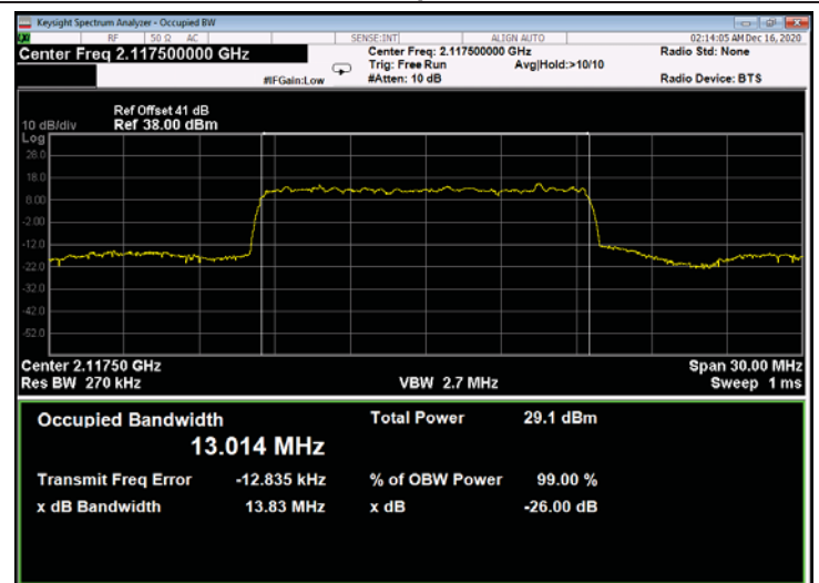
Figure 750: QPSK 15MHz B.W.; 2117.5MHz, 15kHz - Output
