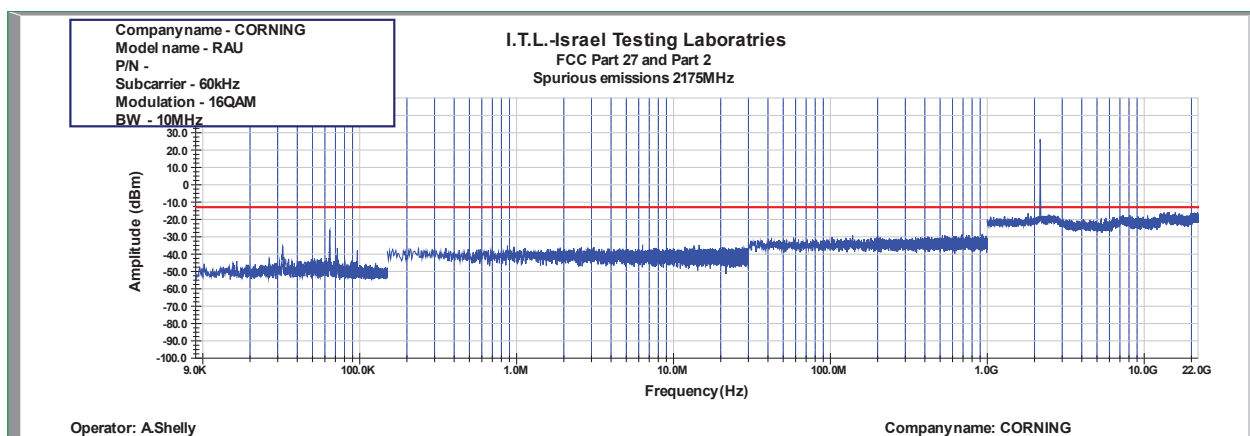
Figure 815: Spurious Emissions at Antenna Terminal 16QAM 10MHz B.W.; 2175.0MHz, 60kHz
