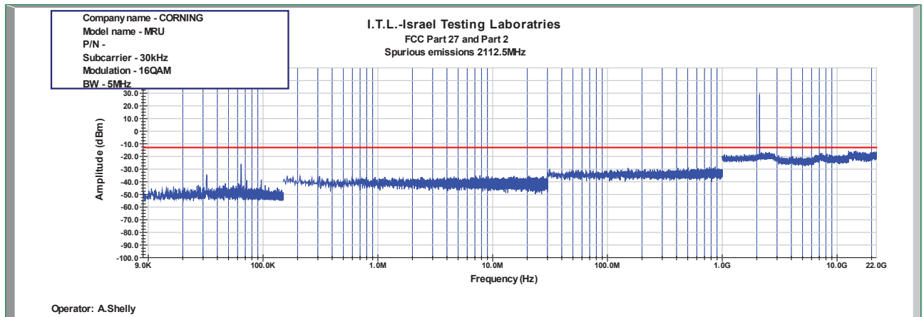
Figure 804: Spurious Emissions at Antenna Terminal 16QAM 5MHz B.W.; 2112.5MHz, 30kHz
