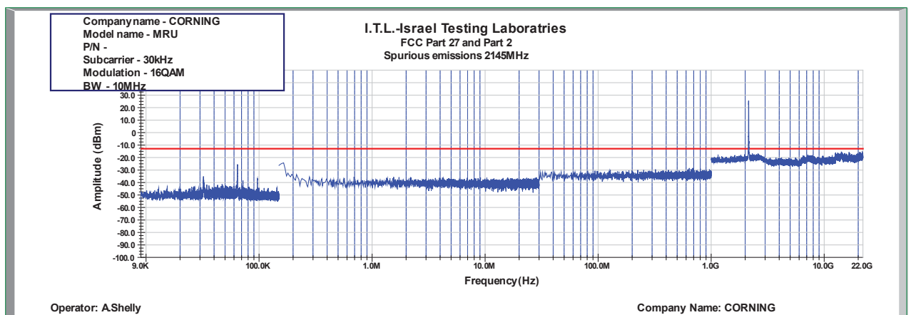
Figure 811: Spurious Emissions at Antenna Terminal 16QAM 10MHz B.W.; 2145.0MHz, 30kHz
