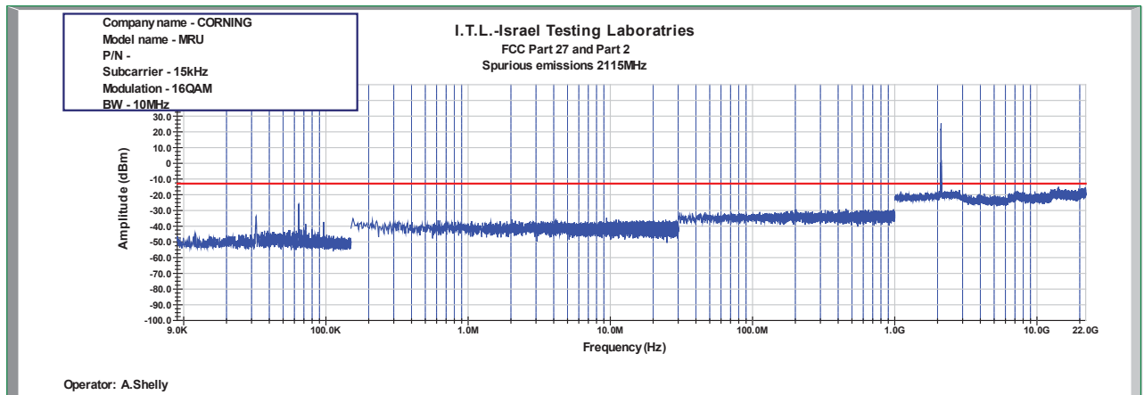
Figure 807: Spurious Emissions at Antenna Terminal 16QAM 10MHz B.W.; 2115.0MHz, 15kHz
