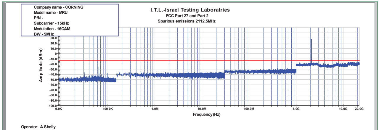
Figure 801: Spurious Emissions at Antenna Terminal 16QAM 5MHz B.W.; 2112.5MHz, 15kHz
