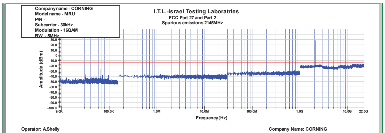
Figure 805: Spurious Emissions at Antenna Terminal 16QAM 5MHz B.W.; 2145.0MHz, 30kHz
