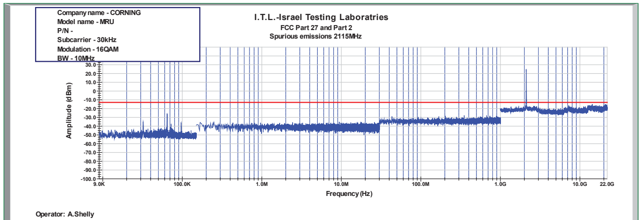
Figure 810: Spurious Emissions at Antenna Terminal 16QAM 10MHz B.W.; 2115.0MHz, 30kHz
