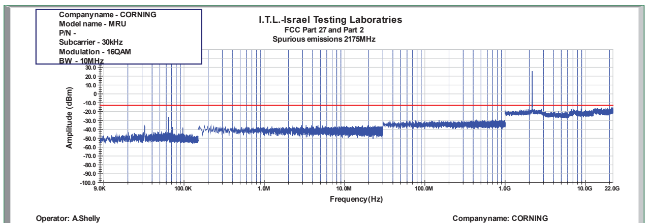
Figure 812: Spurious Emissions at Antenna Terminal 16QAM 10MHz B.W.; 2175.0MHz, 30kHz
