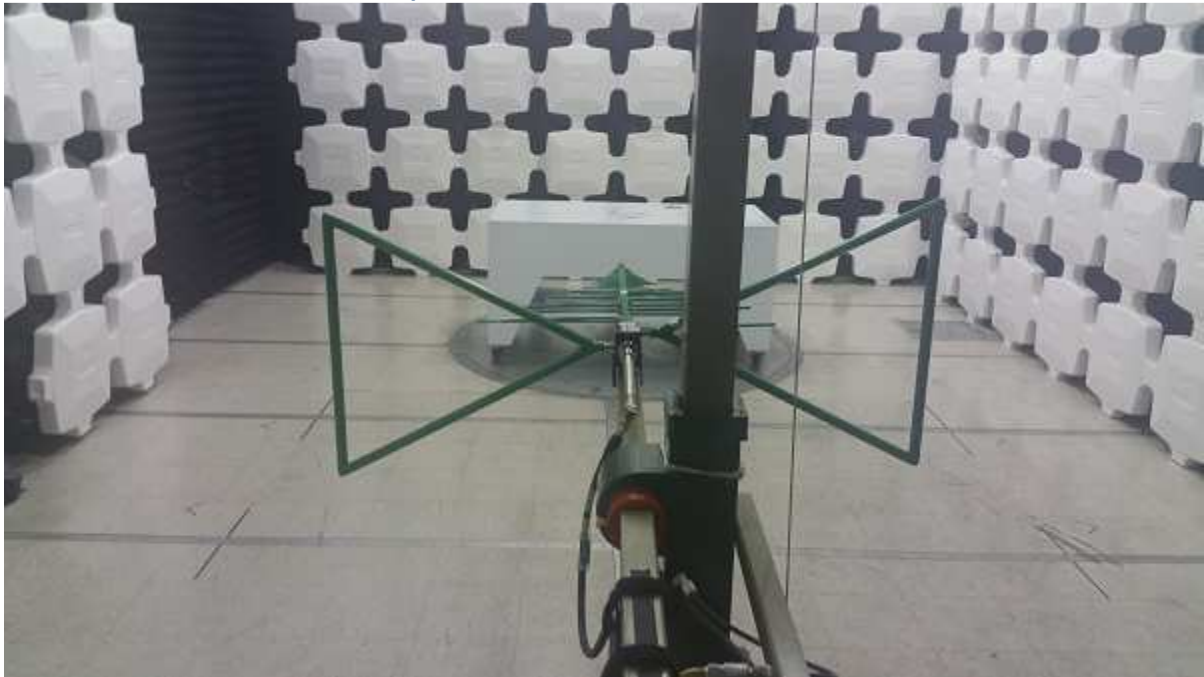
Test setup below 1GHz
