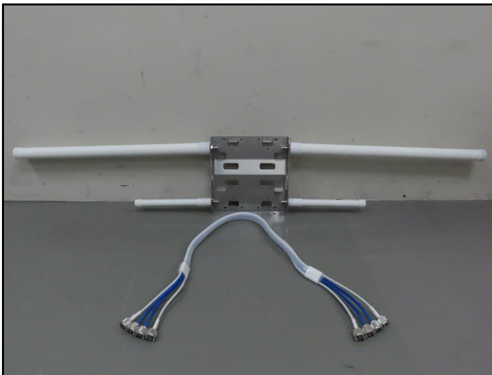
(LoRa/FSK/LTE) Outdoor Antenna
