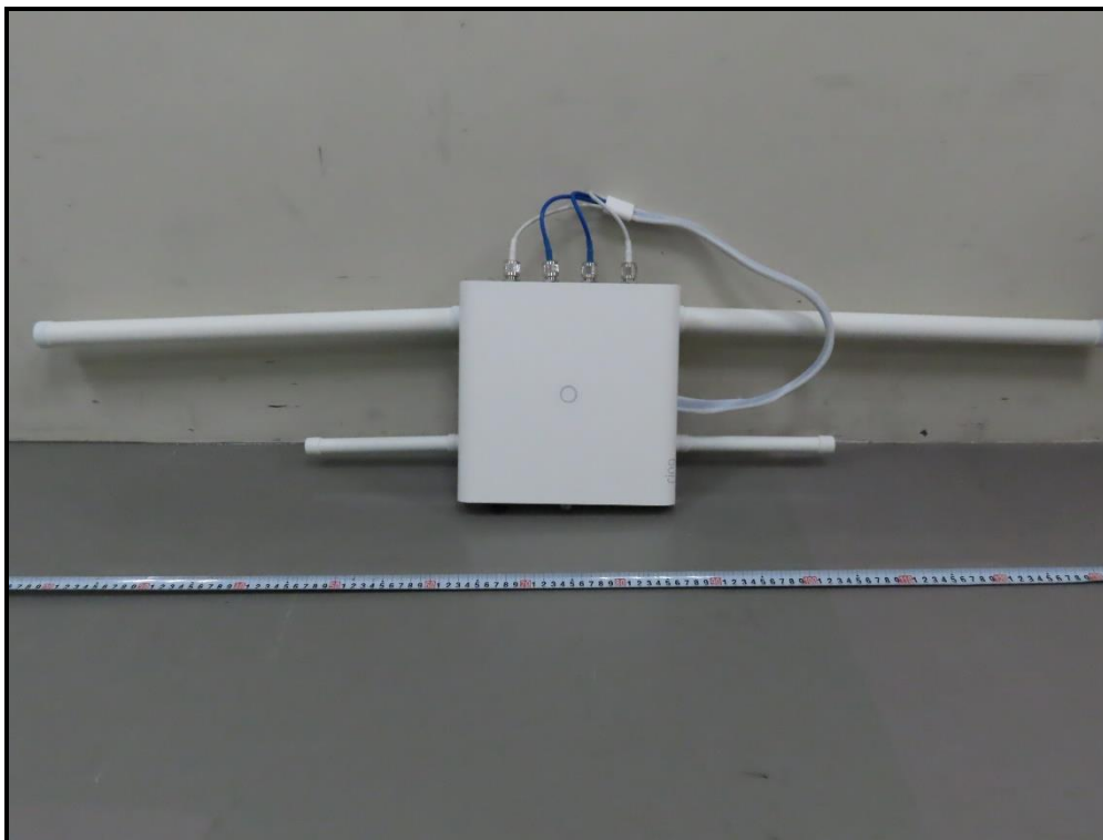
EUT + Outdoor Antenna
