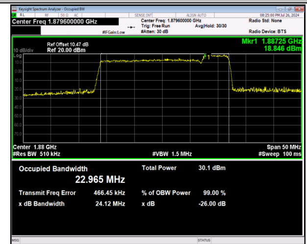
2-2-20MHz-5MHz-64QAM-64QAM-18875-18992-100RB#0 -25RB#0-PASS
