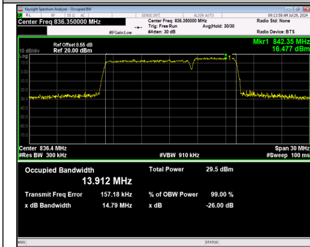
5-5-10MHz-5MHz-64QAM-64QAM-20500-20572-50RB#0-25RB#0-PASS
