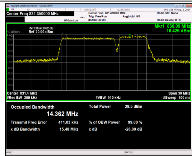
5-5-10MHz-5MHz-QPSK-QPSK-20450-20522-50RB#0-25 RB#0-PASS
