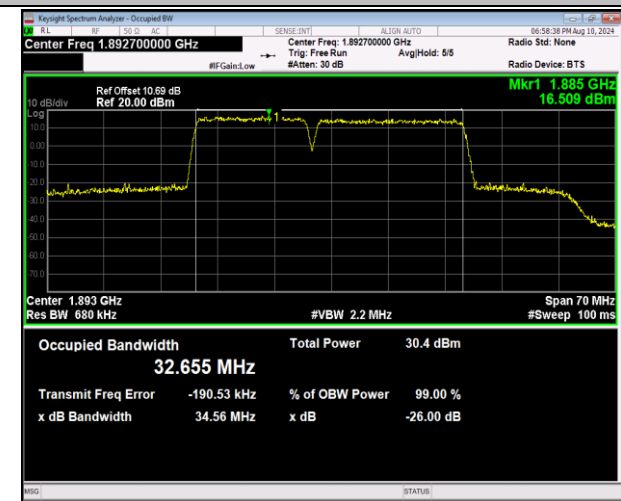
2-2-15MHz-20MHz-QPSK-QPSK-18929-19100-75RB#0-1 00RB#0-PASS
