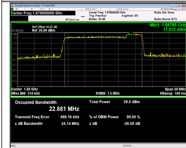
2-2-20MHz-5MHz-16QAM-16QAM-18875-18992-100RB#0 -25RB#0-PASS
