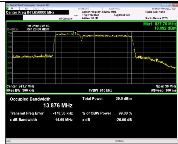
5-5-5MHz-10MHz-16QAM-16QAM-20528-20600-25RB#0-50RB#0-PASS
