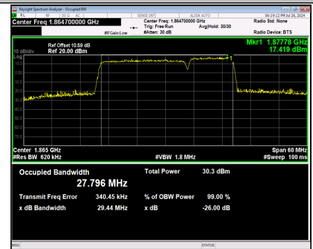
2-2-20MHz-10MHz-64QAM-64QAM-18700-18844-100RB# 0-50RB#0-PASS
