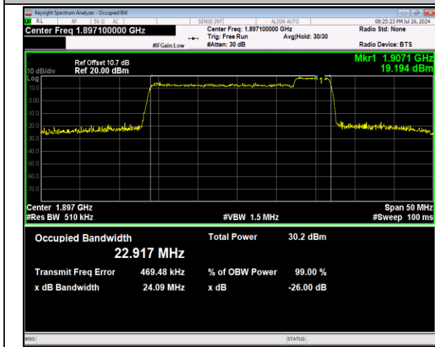
2-2-20MHz-5MHz-64QAM-64QAM-19050-19167-100RB#0 -25RB#0-PASS
