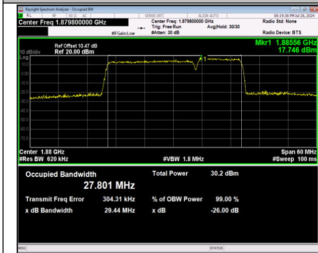
2-2-20MHz-10MHz-64QAM-64QAM-18851-18995-100RB#0-50RB#0-PASS
