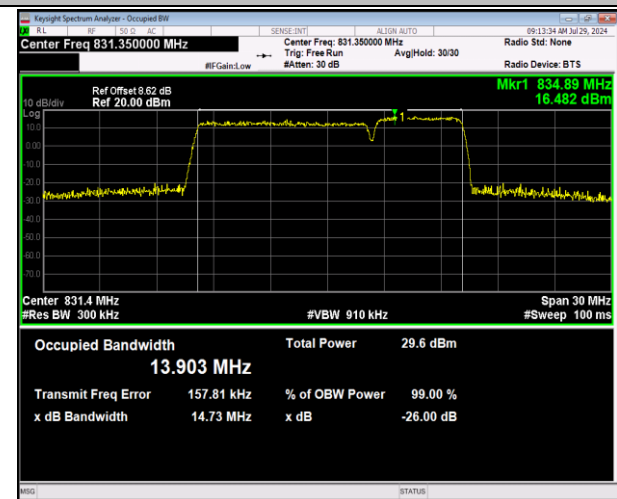
5-5-10MHz-5MHz-64QAM-64QAM-20450-20522-50RB#0-25RB#0-PASS
