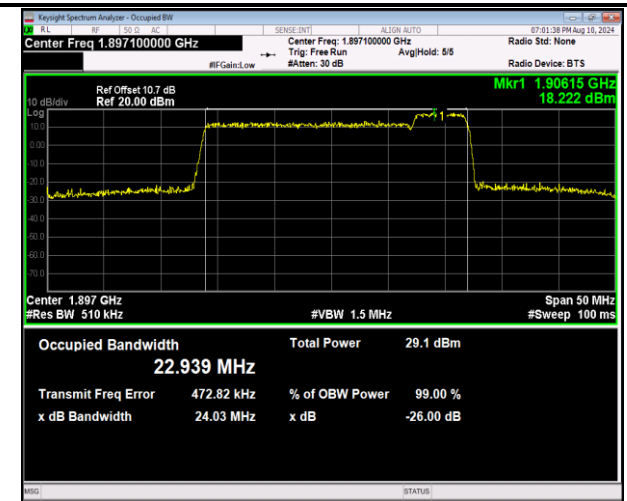
2-2-20MHz-5MHz-16QAM-16QAM-19050-19167-100RB#0 -25RB#0-PASS
