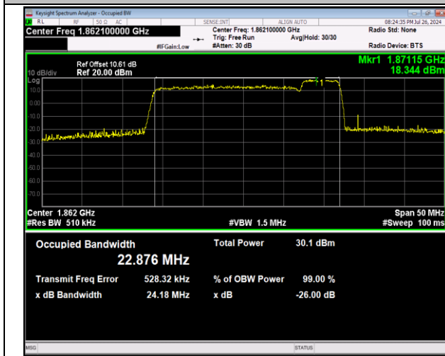
2-2-20MHz-5MHz-64QAM-64QAM-18700-18817-100RB#0 -25RB#0-PASS
