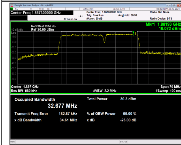
2-2-20MHz-15MHz-64QAM-64QAM-18700-18871-100RB#0-75RB#0-PASS
