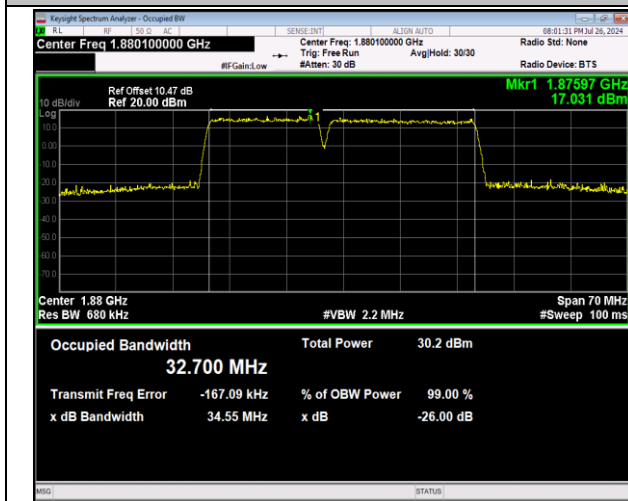
2-2-15MHz-20MHz-64QAM-64QAM-18803-18974-75RB#0 -100RB#0-PASS
