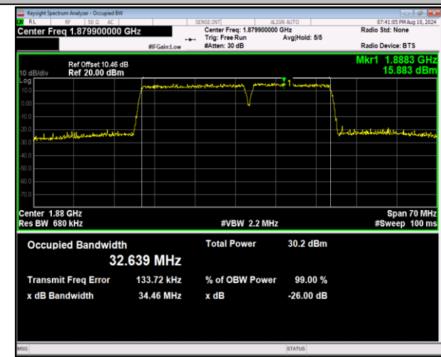
2-2-20MHz-15MHz-QPSK-QPSK-18826-18997-100RB#0-75RB#0-PASS
