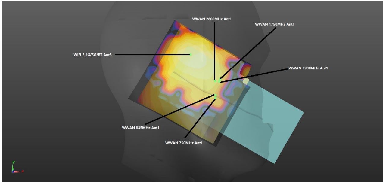
WWAN + WLAN 5GHz/2.4GHz Left Cheek_0mm
