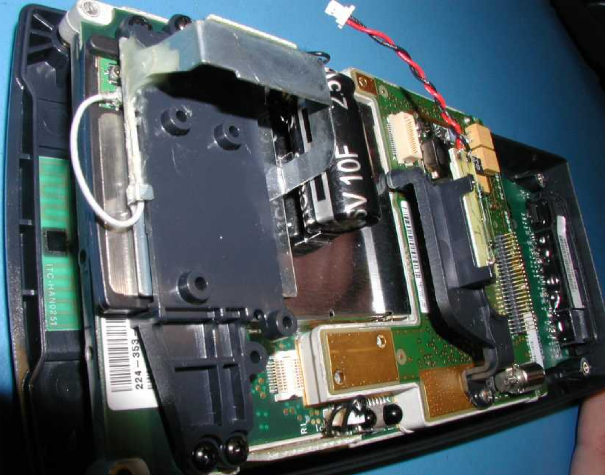
802.11 radio and antenna placement in the 700C
