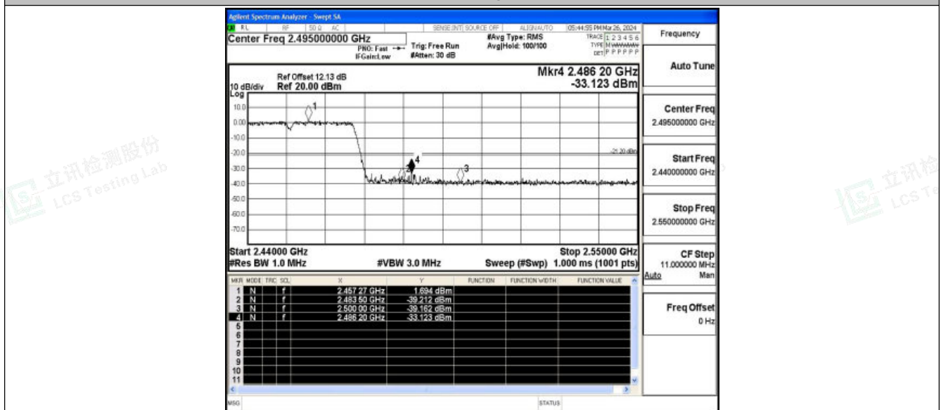
11N40SISO_Ant1_High_2452_Peak
