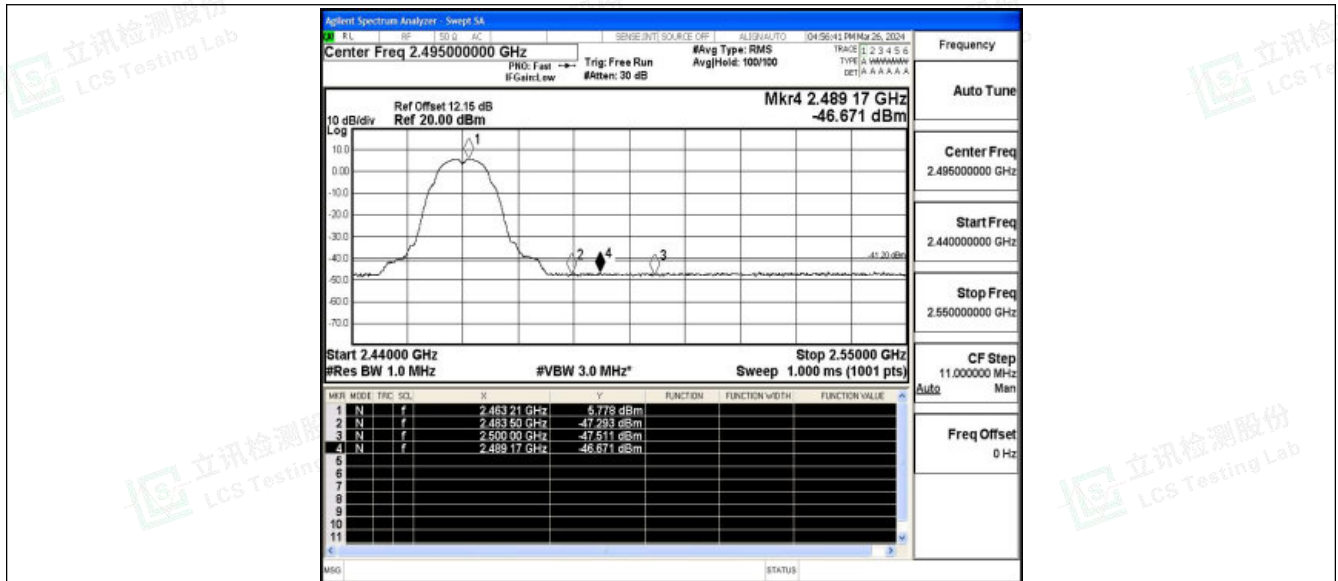
11B_Ant1_High_2462_Peak
