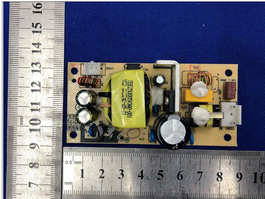
Power board: KC24W07-1002
