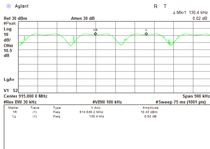
Plot 7.2.1 Carrier frequency separation
