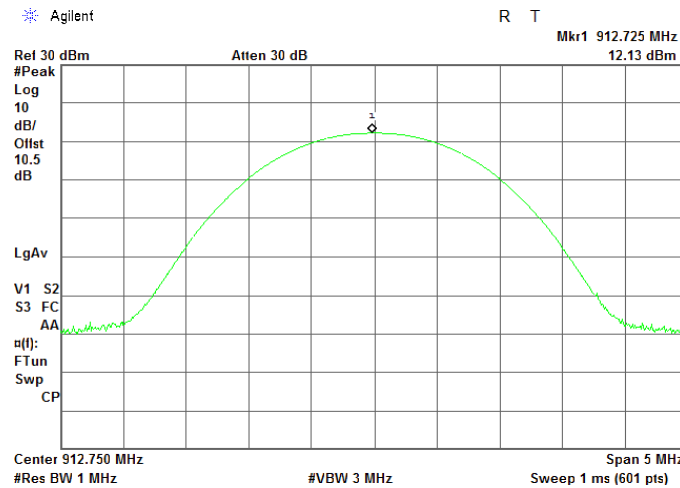
Plot 7.5.1 Peak output power at low frequency
