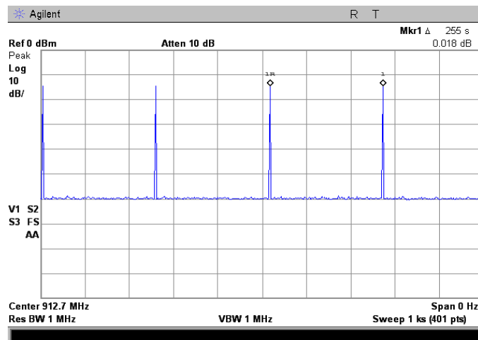
Plot 7.6.9 Single transmission period
