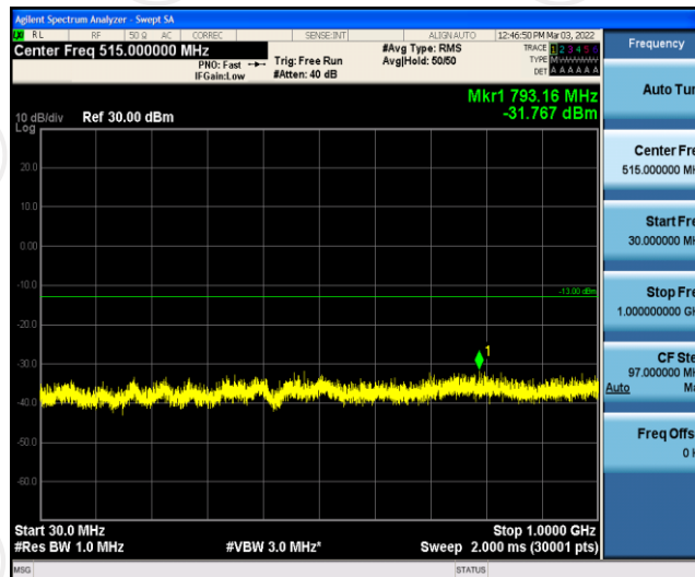
Band4-15MHz-16QAM-20325-1RB#0-Range4:1000~5000MHz
