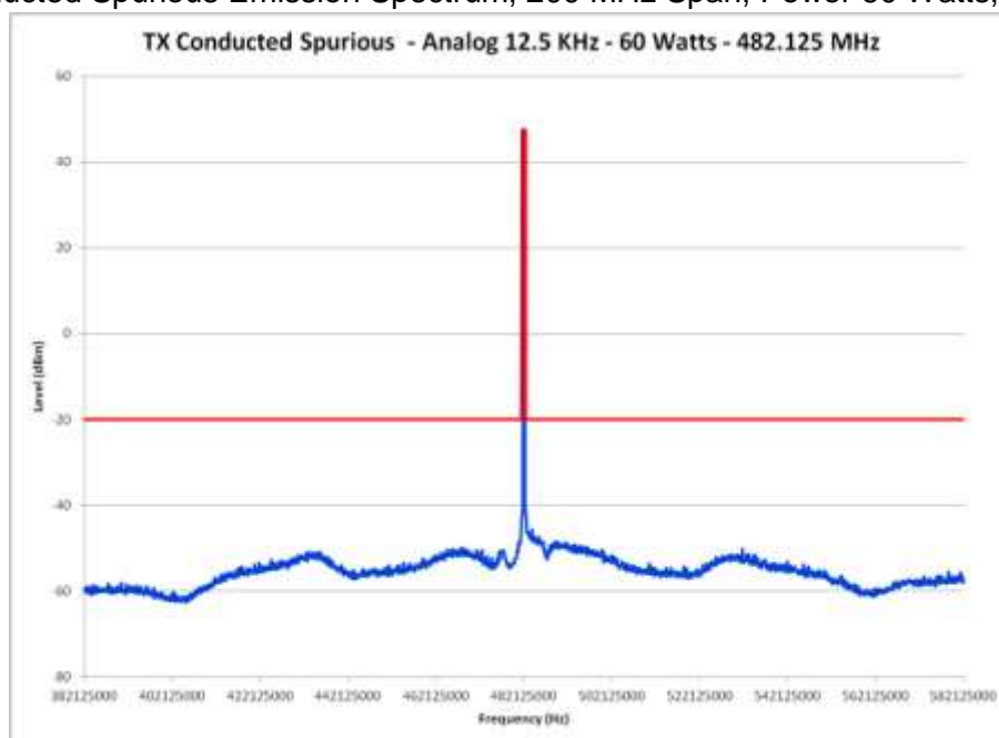
E1-6.6 Conducted Spurious Emission Spectrum, 200 MHz Span, Power 60 Watts, 482.125 MHz
