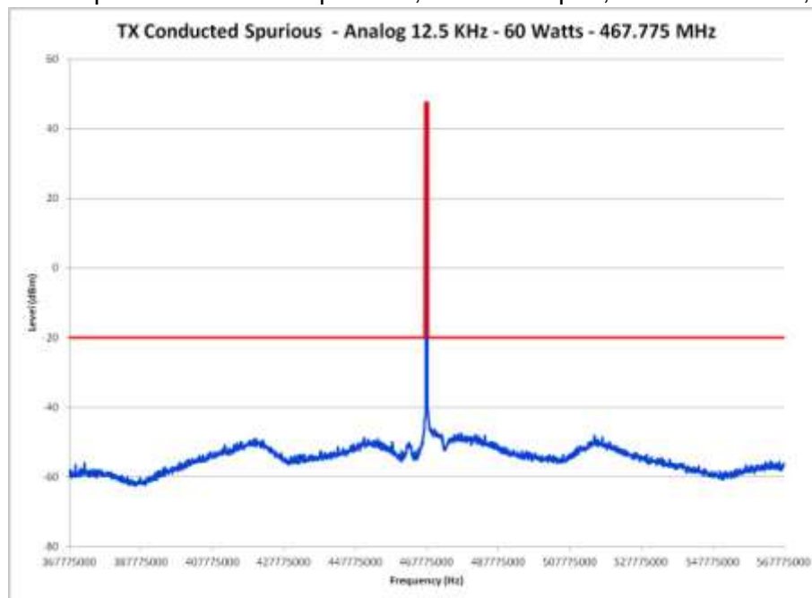
E1-6.5 Conducted Spurious Emission Spectrum, 200 MHz Span, Power 60 Watts, 467.775 MHz
