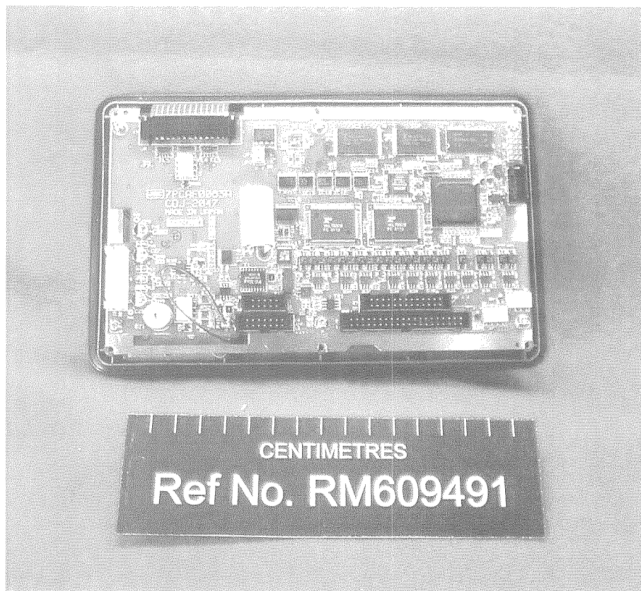
NCM-722 AIS Controller – Internal View 1
