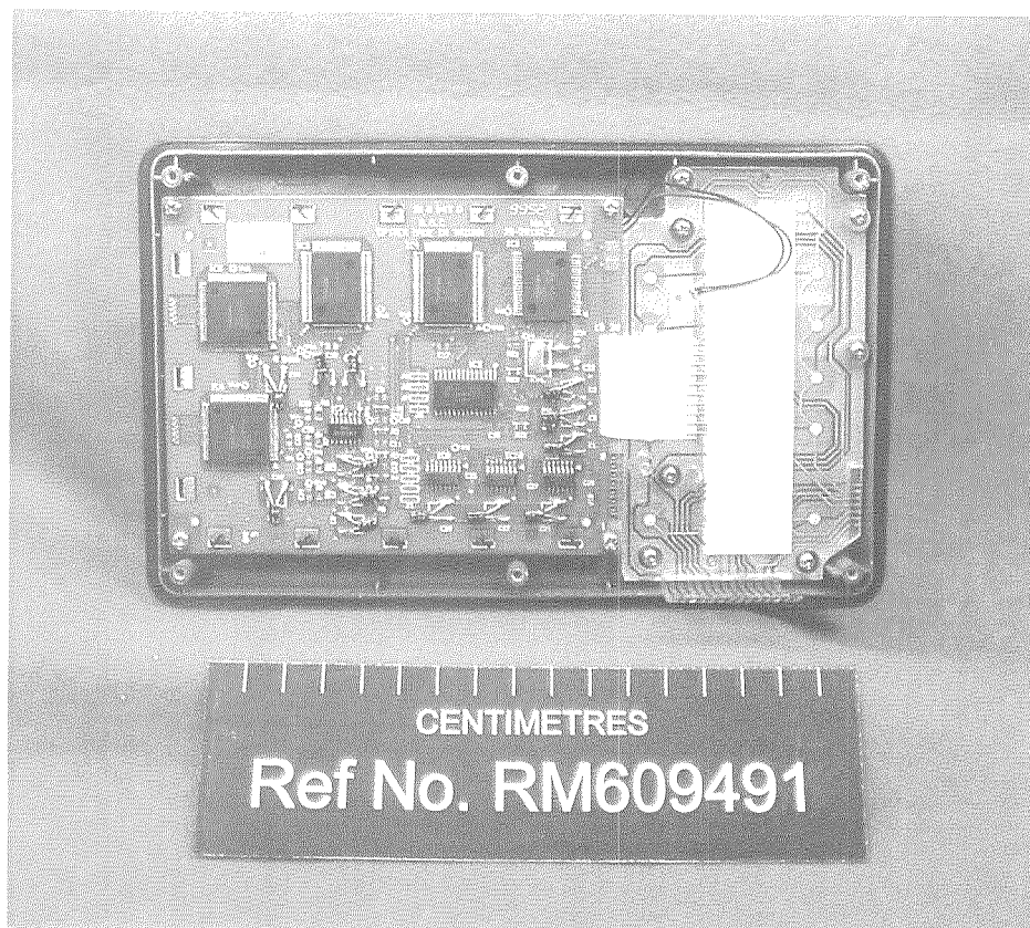
NCM-722 AIS Controller – Internal View 3
