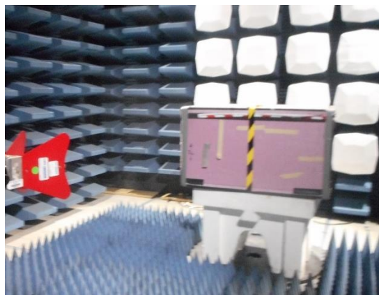
Figure 3: SAC Radiated Spurious Emissions (> 1 GHz) at 3m
