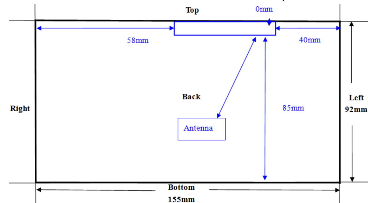
Antenna Configuration 1-Level ( Antenna is folded and align with the edge of EUT )
