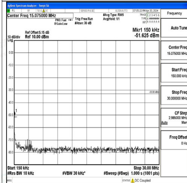
Band66_1.4MHz_16QAM_131979_1RB#0_0.15~30_0.15~30
