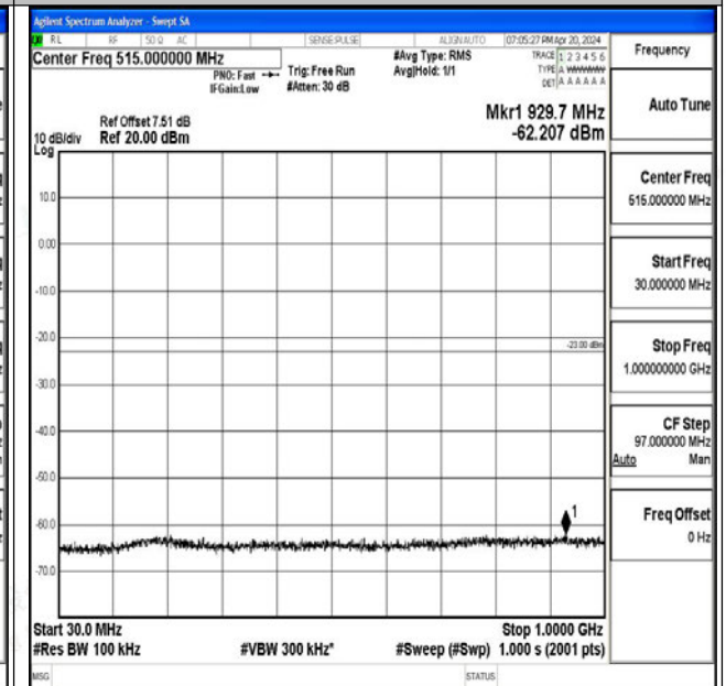
Band66_1.4MHz_16QAM_131979_1RB#0_30~1000_30~1000
