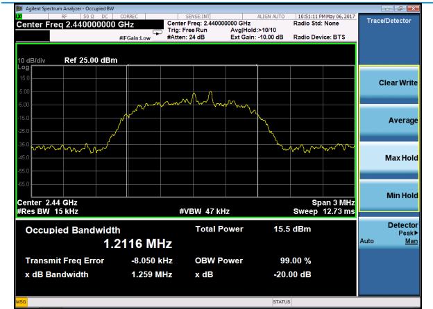
EDR3 – Mid Channel
