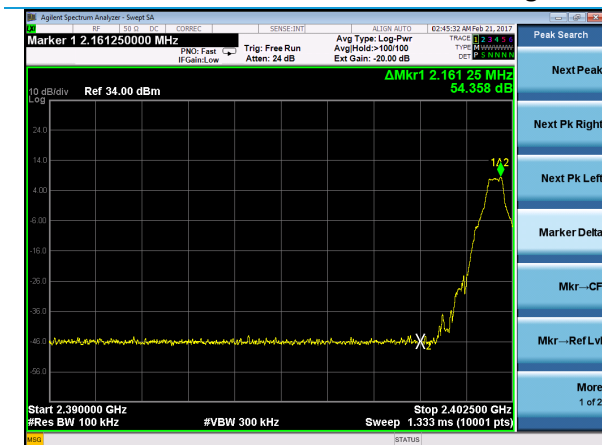
GFSK – Hopping – Lower Band Edge
