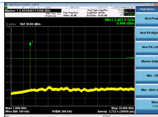
Low Channel – 1-10 GHz
