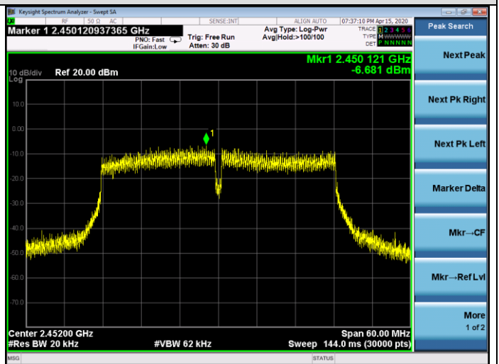
11nHT40-HCH
