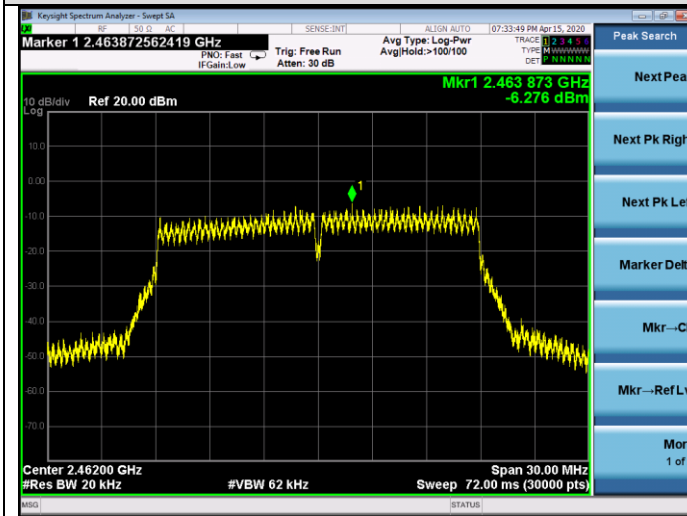
11nHT20-HCH
