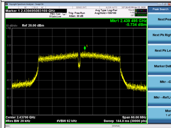
11nHT40-MCH
