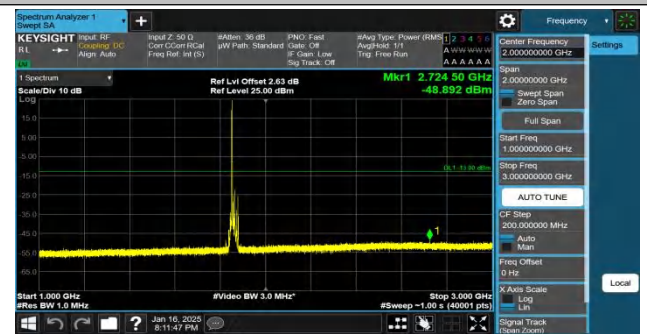
Band2-15MHz-QPSK-18675-1RB#0-1000~3000-PASS
