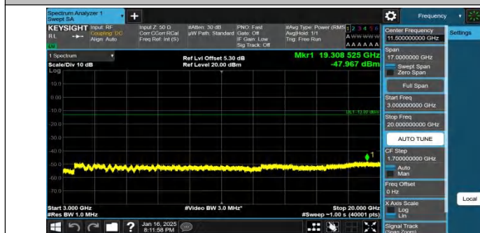
Band2-15MHz-QPSK-18675-1RB#0-3000~20000-PASS
