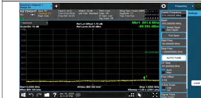
Band2-15MHz-QPSK-18675-1RB#0-30~1000-PASS
