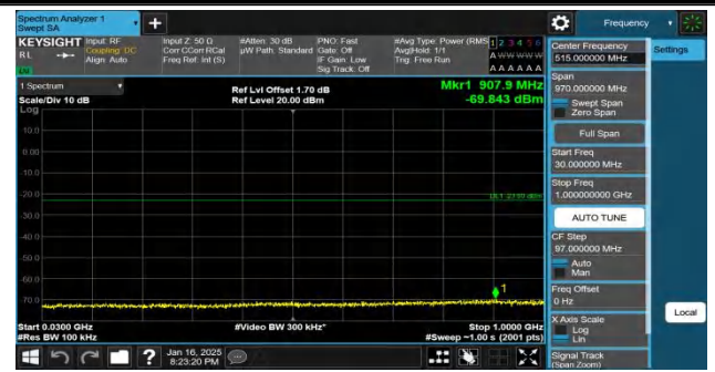
Band2-20MHz-QPSK-19100-1RB#99-30~1000-PASS
