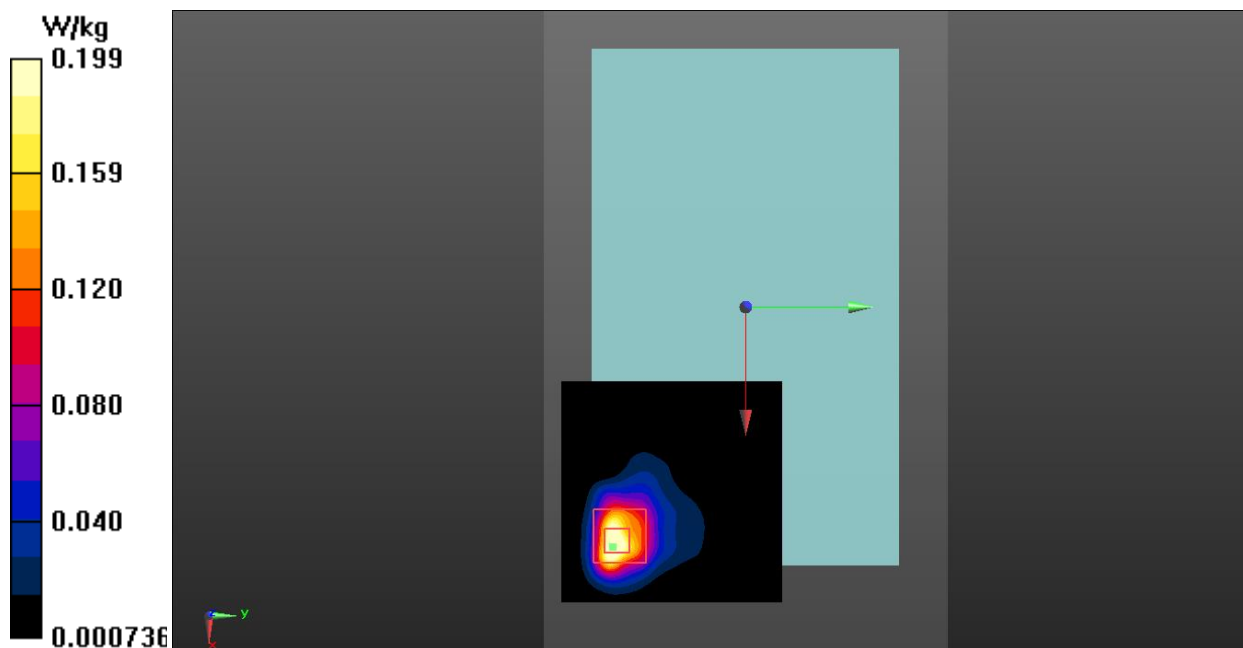
Fig. 13 Bluetooth Body
