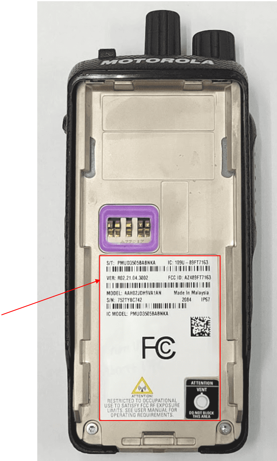
Back View (FCC/IC Label Location) for Limited Keypad and Non-Keypad Model
