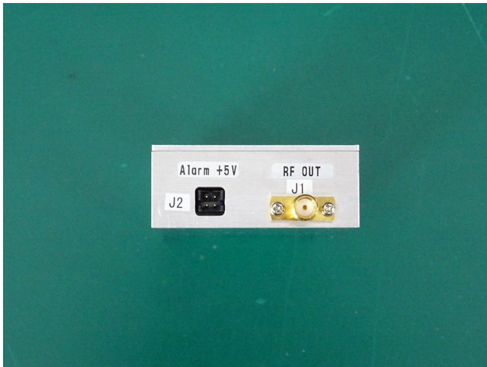
Oscillator Module (2 nd Local/CGH-382A) Connector side view
