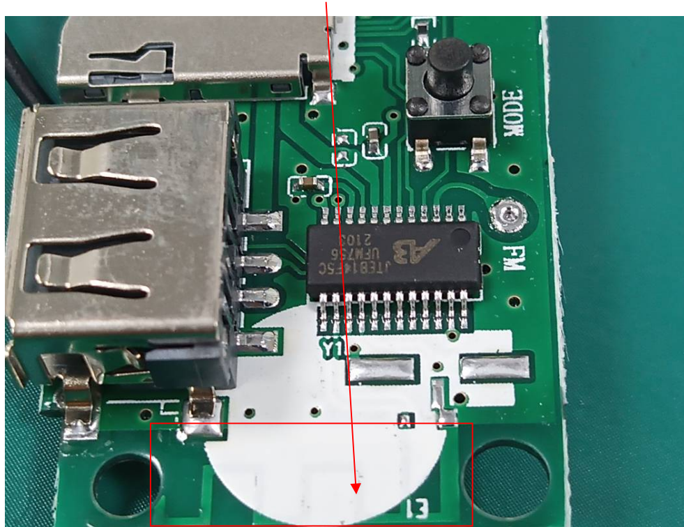
Bluetooth Antenna
