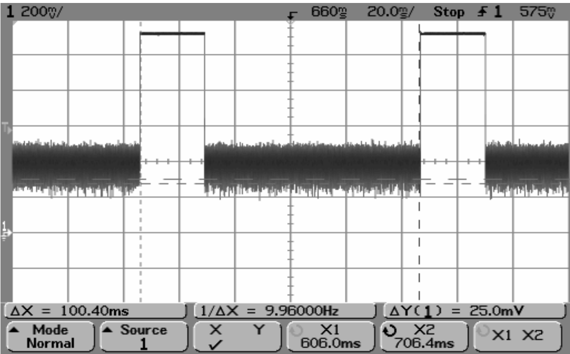
SP-652-XXX: Number of Data Pulses in 100 msec period
