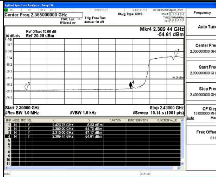
11N40SISO_Ant1_Low_2422_Peak
