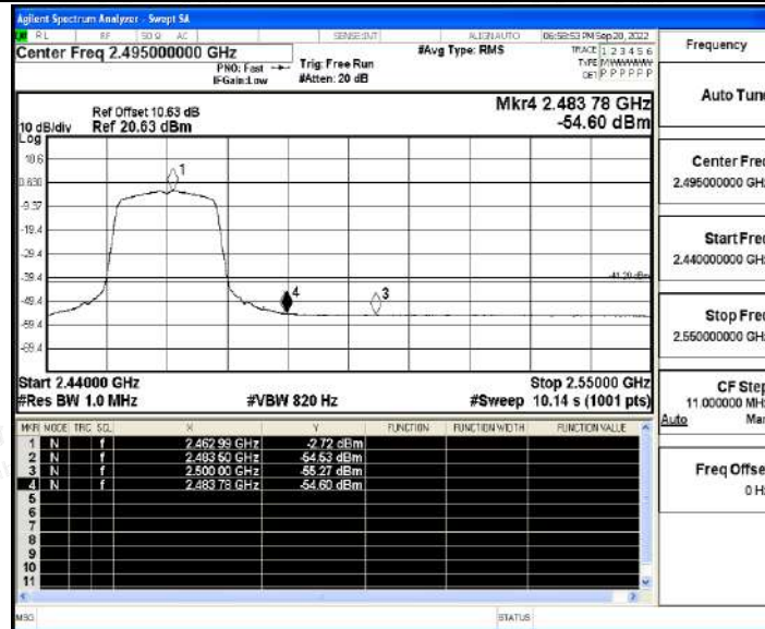
11N20ISO_Ant1_High_2462_Peak
