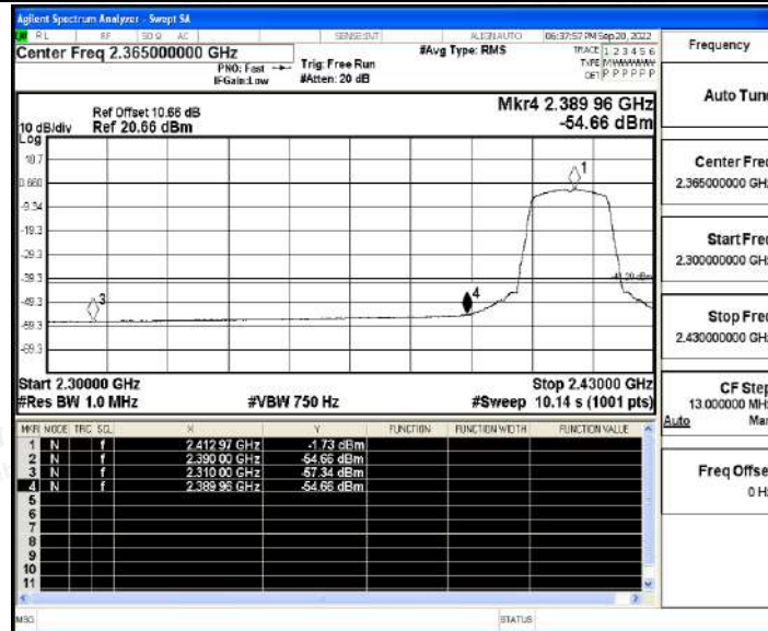
11G_Ant1_Low_2412_Peak
