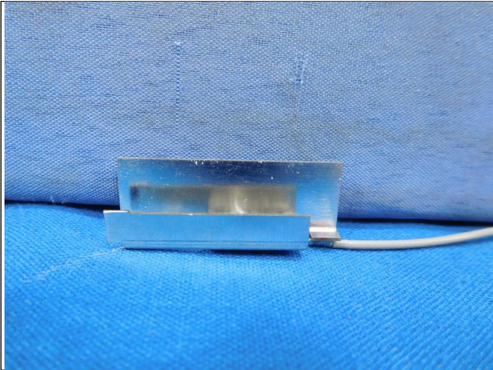
Antenna - 2.4GHz chain 0
