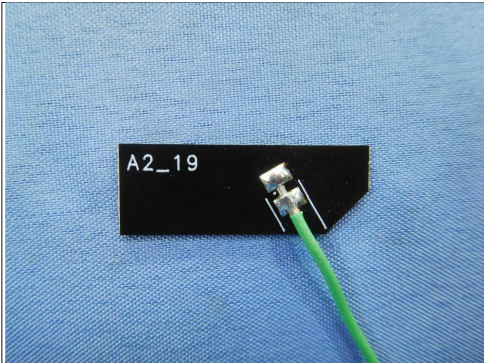
Antenna - 5GHz chain 0
