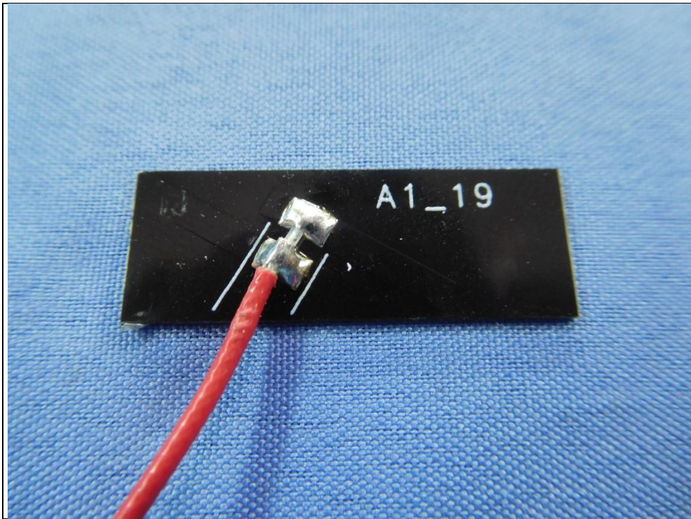
Antenna - 5GHz chain 1
