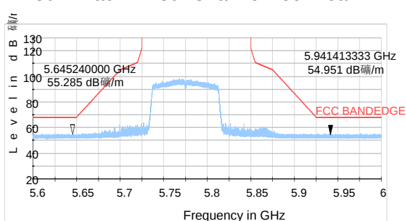
802.11ac VHT80- Channel 155: Peak
