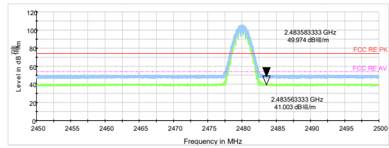
DH5-Channel 78: Peak & Average
