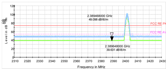
3DH5-Channel 0: Peak & Average
