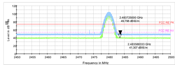
3DH5-Channel 78: Peak & Average
