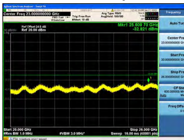
Band7-20G-26G / 15MHz / High CH / 64QAM
