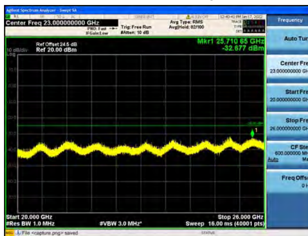
Band7-20G-26G / 15MHz / High CH / 16QAM
