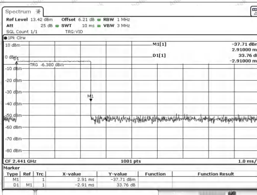
Dwell_Time_(Hopping)_NVNT_ANT1_1-DH5_2441_One_Burst_Time
