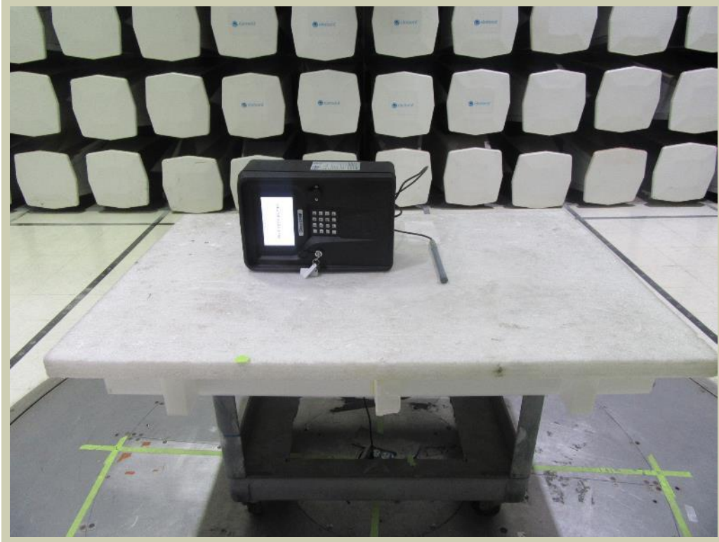
FIELD STRENGTH OF SPURIOUS EMISSIONS (LESS THAN 30 MHz)
