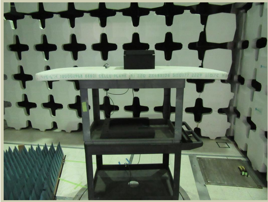
FIELD STRENGTH OF SPURIOUS EMISSIONS (Above 1GHz)
