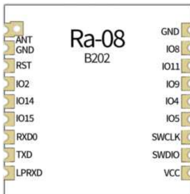
Figure 5 Schematic diagram of module pins
