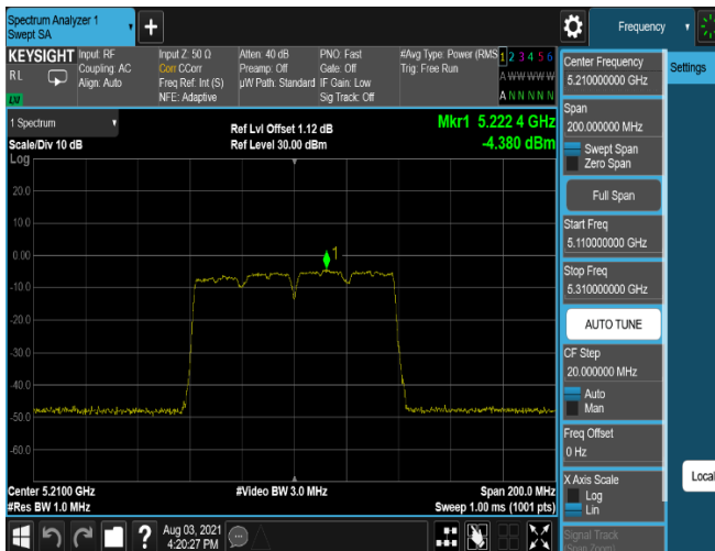
Plot 7-663. ISED PSD SDM Antenna 5T (80MHz BW 11ac – Ch.42, MCS5)
