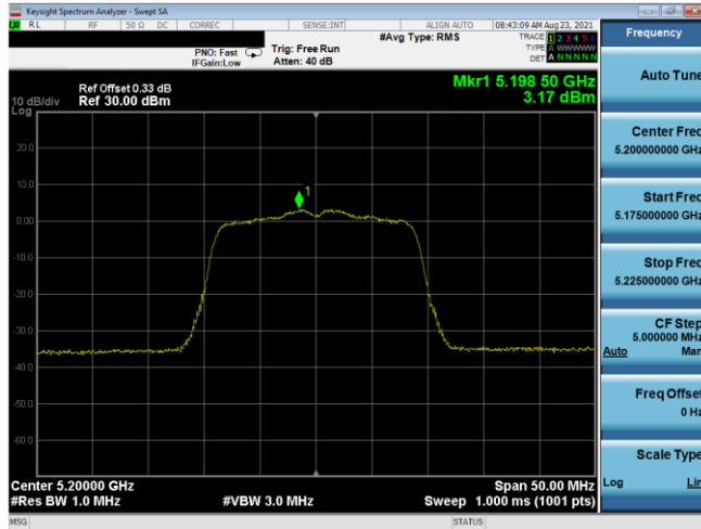
Plot 7-643. ISED PSD SDM Antenna 5T (20MHz BW 11n – Ch.40, MCS11)
