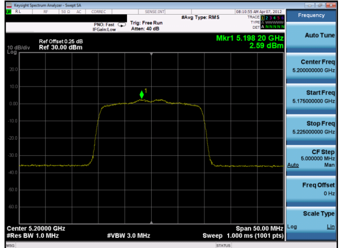
Plot 7-646. ISED PSD SDM Antenna 3b (20MHz BW 11ax(SU) – Ch.40, MCS3)
