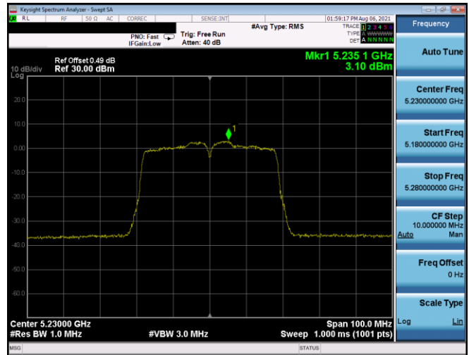
Plot 7-635. ISCED PSD SDM Antenna 5T (40MHz BW 11n – Ch.46, MCS10)
