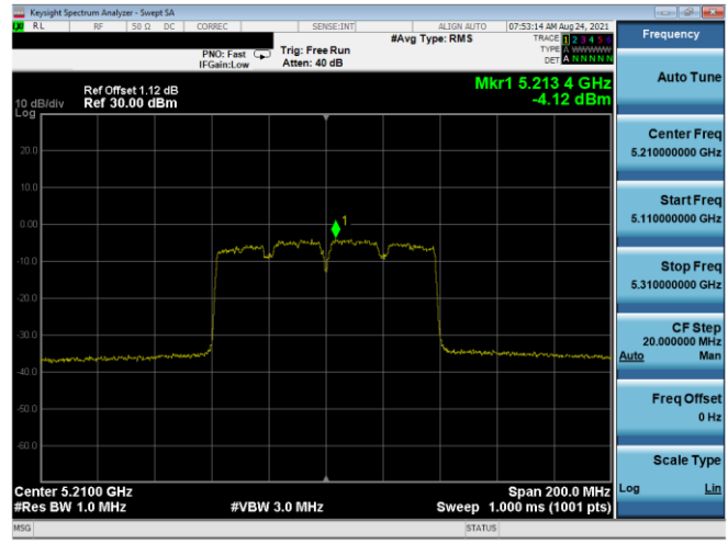
Plot 7-664. ISED PSD SDM Antenna 3b (80MHz BW 11ac – Ch.42, MCS5)
