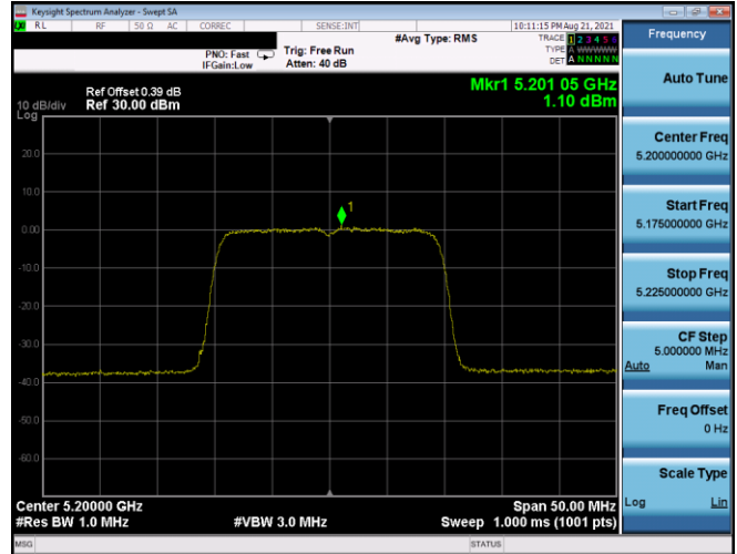
Plot 7-658. ISED PSD SDM Antenna 3b (20MHz BW 11ax(SU) - Ch.40, MCS11)
