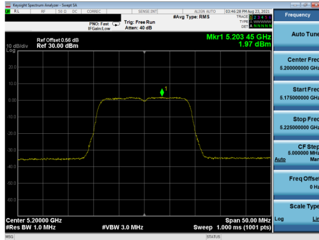
Plot 7-655. ISED PSD SDM Antenna 5T (20MHz BW 11n - Ch.40, MCS13)
