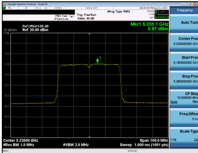
Plot 7-661. ISED PSD SDM Antenna 5T (40MHz BW 11ax(SU) – Ch.46, MCS11)
