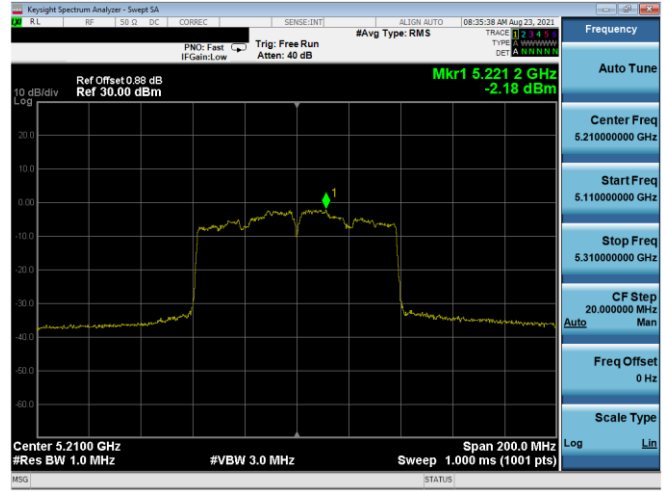
Plot 7-652. ISED PSD SDM Antenna 3b (80MHz BW 11ac – Ch.42, MCS3)
