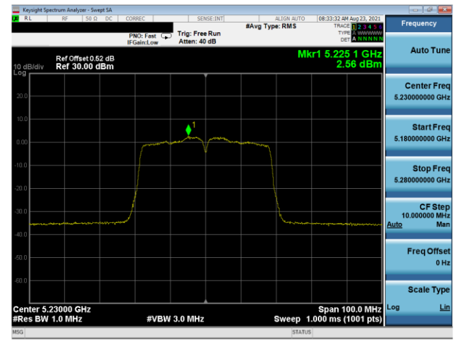
Plot 7-648. ISED PSD SDM Antenna 3b (40MHz BW 11n – Ch.46, MCS11)
