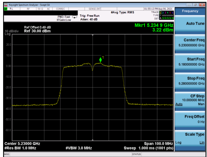
Plot 7-636. ISCED PSD SDM Antenna 3b (40MHz BW 11n – Ch.46, MCS10)
