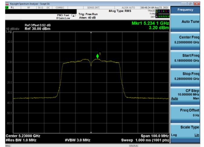
Plot 7-647. ISED PSD SDM Antenna 5T (40MHz BW 11n – Ch.46, MCS11)
