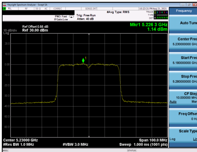
Plot 7-662. ISED PSD SDM Antenna 3b (40MHz BW 11ax(SU) – Ch.46, MCS11)
