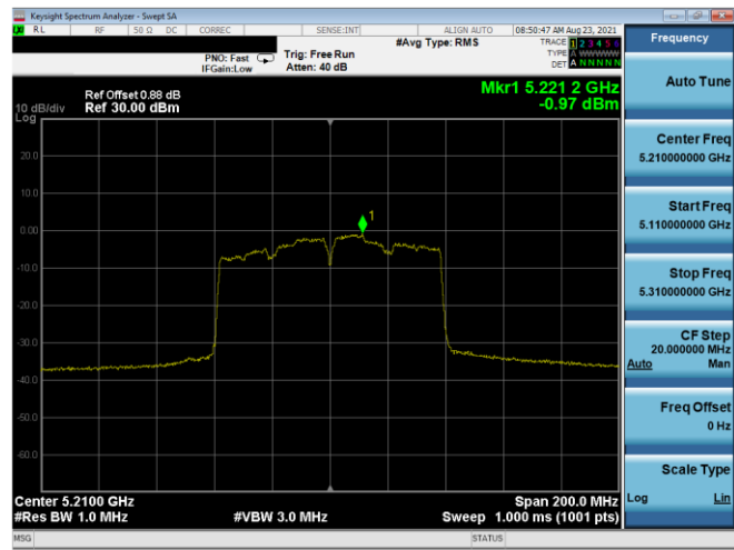
Plot 7-651. ISED PSD SDM Antenna 5T (80MHz BW 11ac – Ch.42, MCS3)
