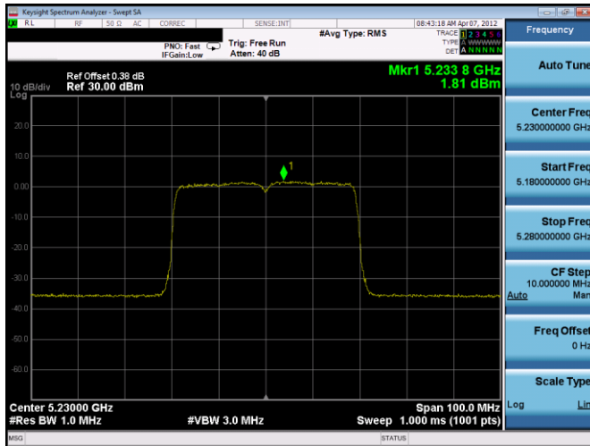
Plot 7-649. ISED PSD SDM Antenna 5T (40MHz BW 11ax(SU) – Ch.46, MCS3)
