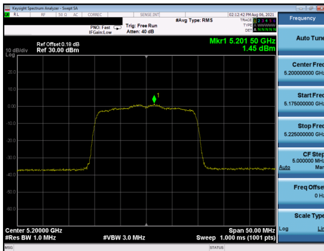
Plot 7-633. ISCED PSD SDM Antenna 5T (20MHz BW 11ax(SU) – Ch.40, MCS2)
