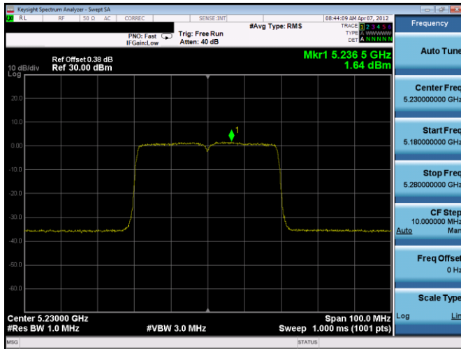
Plot 7-650. ISED PSD SDM Antenna 3b (40MHz BW 11ax(SU) – Ch.46, MCS3)
