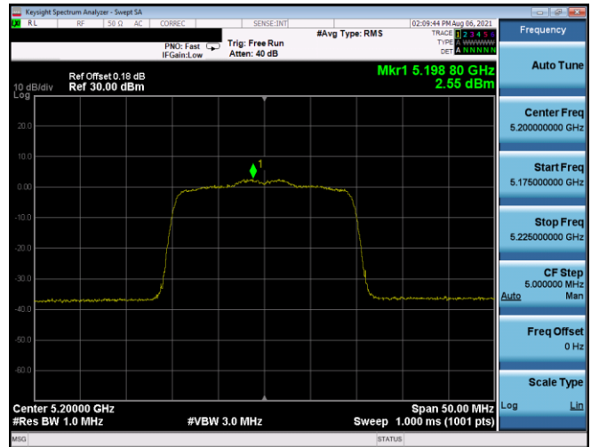
Plot 7-634. ISCED PSD SDM Antenna 3b (20MHz BW 11ax(SU) – Ch.40, MCS2)
