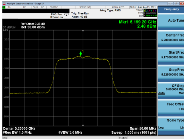
Plot 7-644. ISED PSD SDM Antenna 3b (20MHz BW 11n – Ch.40, MCS11)
