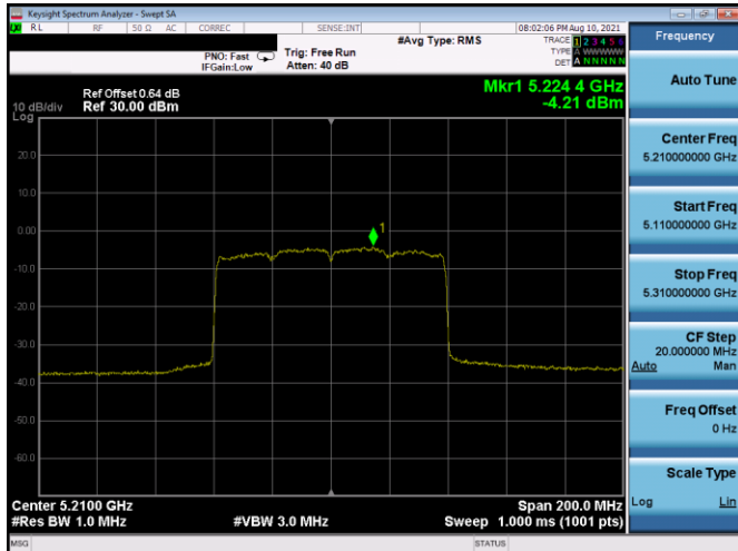
Plot 7-654. ISED PSD SDM Antenna 3b (80MHz BW 11ax (SU) – Ch.42, MCS3)
