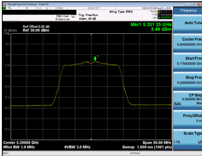
Plot 7-631. ISCED PSD SDM Antenna 5T (20MHz BW 11n – Ch.40, MCS10)
