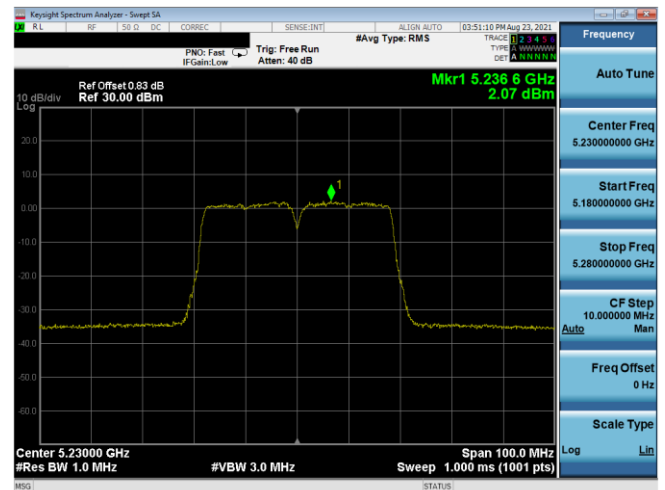
Plot 7-659. ISED PSD SDM Antenna 5T (40MHz BW 11n - Ch.46, MCS13)
