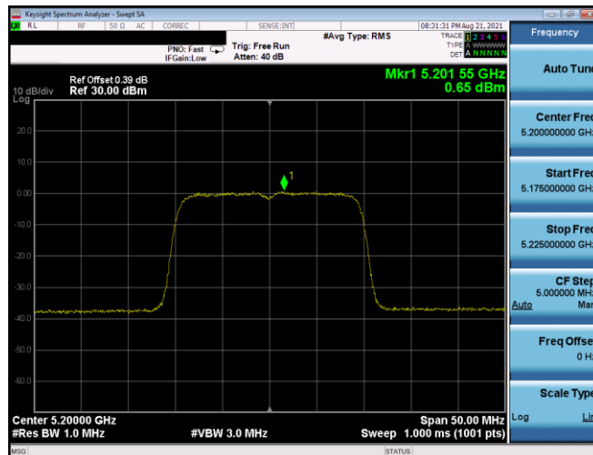
Plot 7-657. ISED PSD SDM Antenna 5T (20MHz BW 11ax(SU) - Ch.40, MCS11)
