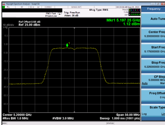
Plot 7-656. ISED PSD SDM Antenna 3b (20MHz BW 11n - Ch.40, MCS13)
