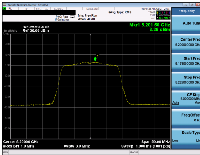
Plot 7-632. ISCED PSD SDM Antenna 3b (20MHz BW 11n – Ch.40, MCS10)
