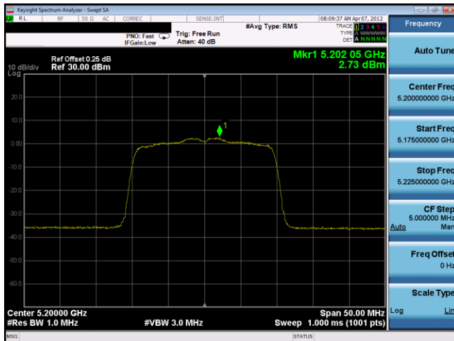
Plot 7-645. ISED PSD SDM Antenna 5T (20MHz BW 11ax(SU) – Ch.40, MCS3)
