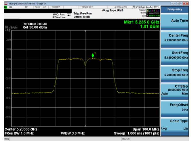
Plot 7-660. ISED PSD SDM Antenna 3b (40MHz BW 11n - Ch.46, MCS13)
