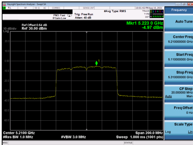
Plot 7-653. ISED PSD SDM Antenna 5T (80MHz BW 11ax (SU) – Ch.42, MCS3)
