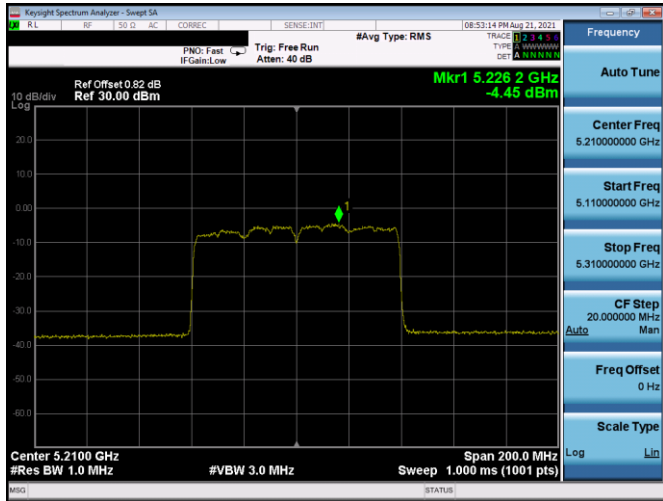
Plot 7-665. ISED PSD SDM Antenna 5T (80MHz BW 11ax(SU) – Ch.42, MCS11)
