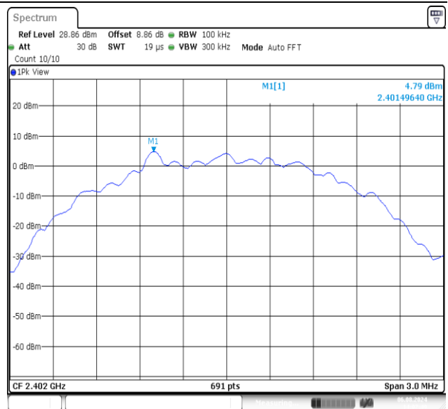
BLE_2M-Ant1-2402-0~Reference-PASS
