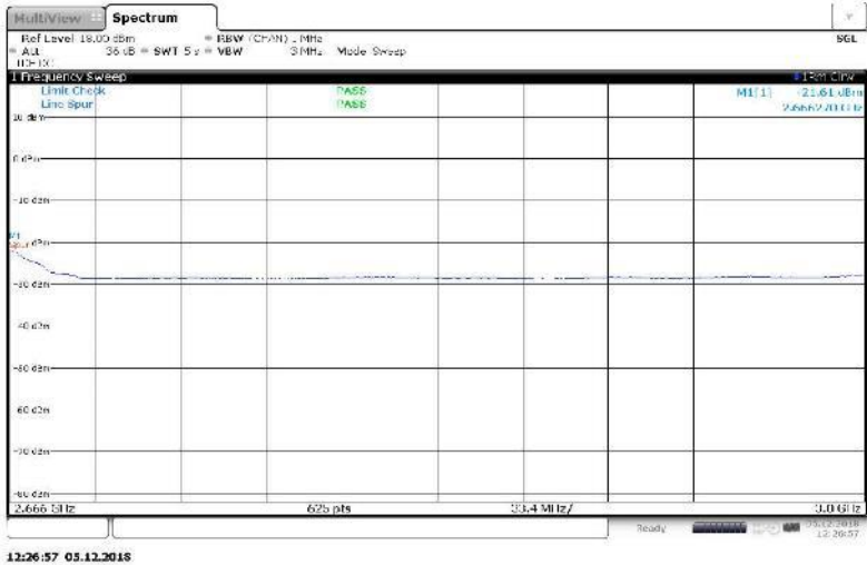
Figure 84 Spurious Emissions (2.666 GHz – 3 GHz) – 16QAM (2655 MHz, 20 MHz Channel BW)
