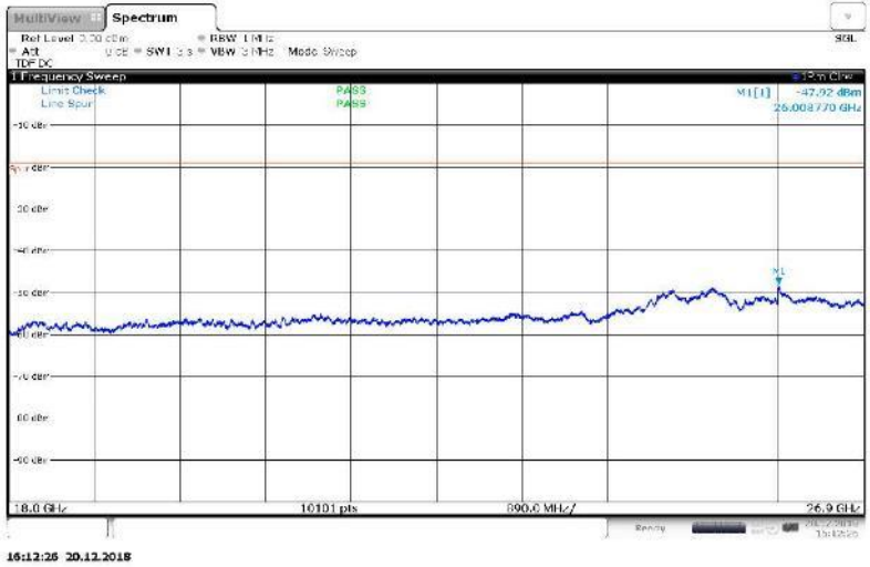
Figure 92 Spurious Emissions (18GHz – 26.9GHz) – 64QAM (2655 MHz, 20 MHz Channel BW)
