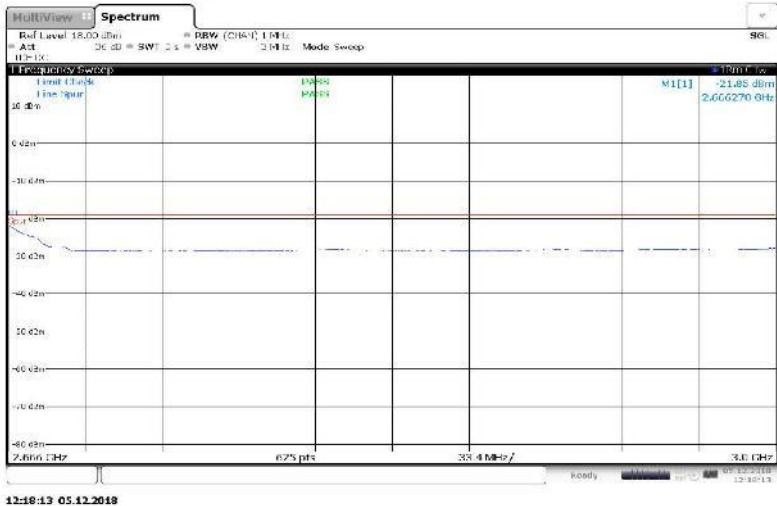
Figure 90 Spurious Emissions (2.666 GHz – 3 GHz) – 64QAM (2655 MHz, 20 MHz Channel BW)
