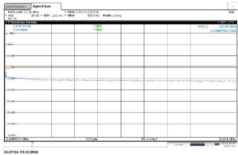
Figure 64 Spurious Emissions (Upper Band Edge) – 64QAM (2682.5 MHz, 15 MHz Channel BW)
