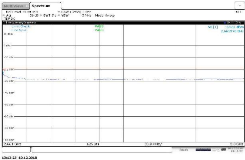
Figure 108 Spurious Emissions (2.661 GHz – 3 GHz) – 16QAM (2652.5 MHz, 2657.5 MHz, 2x5 Channel BW)
