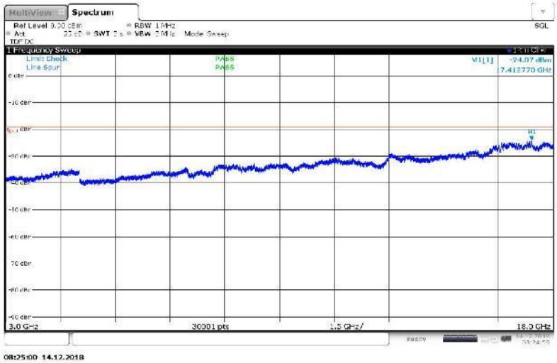
Figure 91 Spurious Emissions (3 GHz – 18GHz) – 64QAM (2655 MHz, 20 MHz Channel BW)
