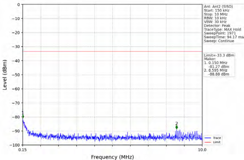
802.11ax(HEW20)_LCH_2412MHz_SU_Ant2 (SISO)_NTNV
