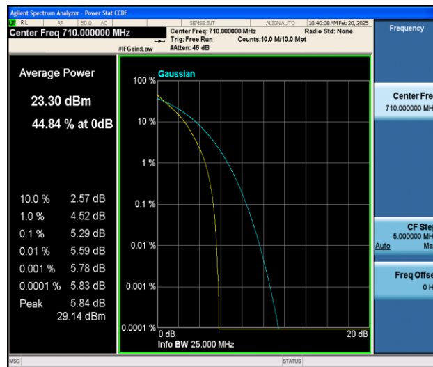
Band17-5MHz-QPSK-23790-25RB#0-PASS
