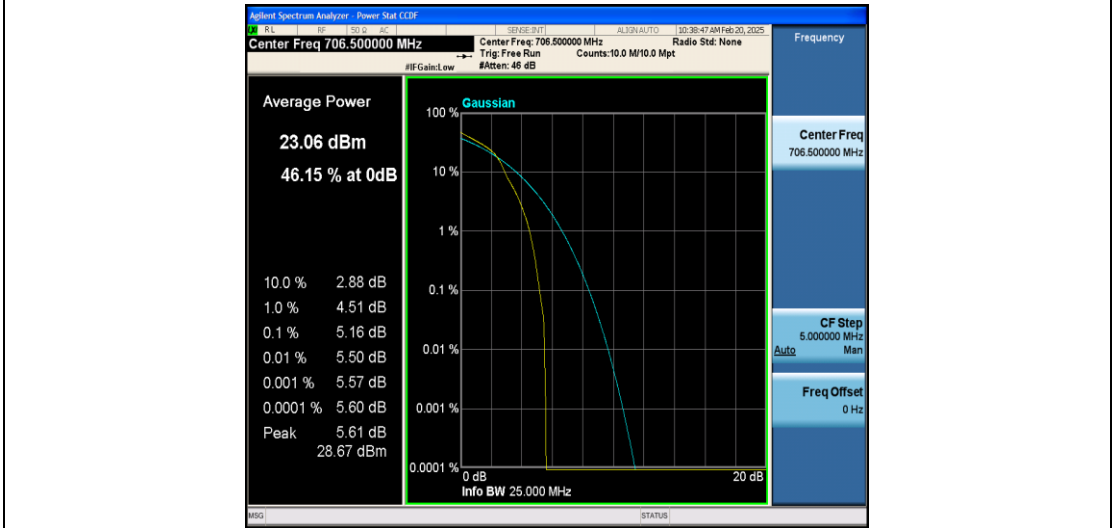
Band17-5MHz-16QAM-23755-1RB#0-PASS
