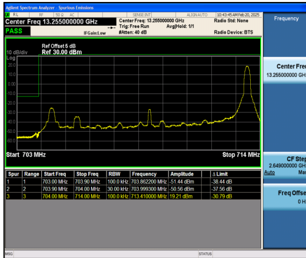
Band17_10MHz_16QAM_23780_1RB#49
