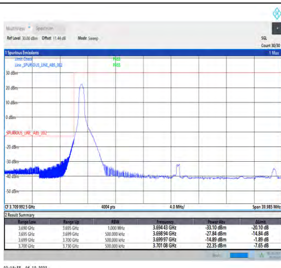
1-N77-3700-3980-PC2-30-30-L-1-DFT-QPSK-Edge_1 RB_Left-1@0-Ant1-1--PASS-see graph
