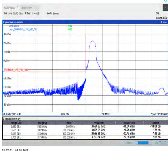
1-N77-3700-3980-PC2-30-10-L-1-DFT-QPSK-Edge_1 RB_Left-1@0-Ant1-1--PASS-see graph
