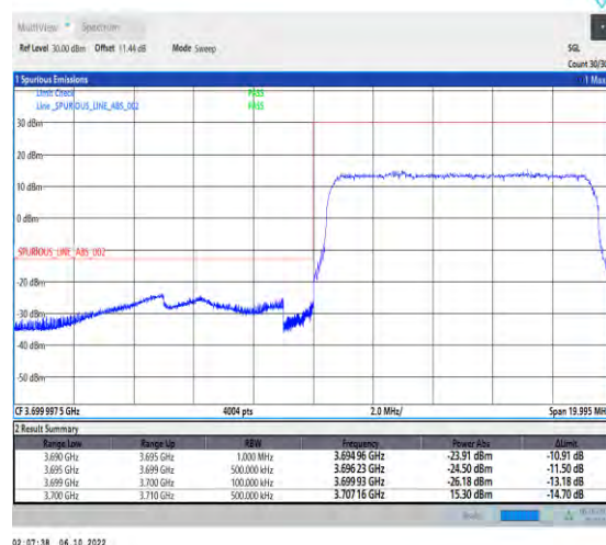
1-N77-3700-3980-PC2-30-10-L-3-DFT-QPSK-Outer_Full-24@0-Ant1-1--PASS-see graph
