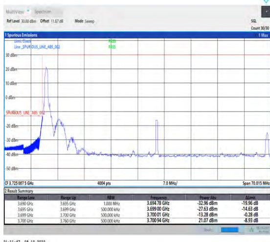
1-N77-3700-3980-PC2-30-60-L-1-DFT-QPSK-Edge_1 RB_Left-1@0-Ant1-1--PASS-see graph
