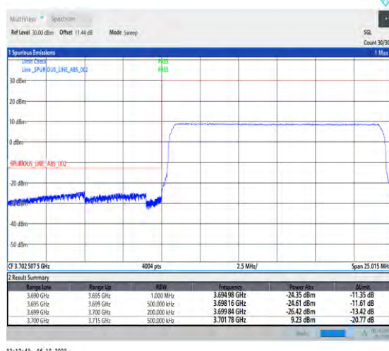
1-N77-3700-3980-PC2-30-15-L-6-CP-QPSK-Outer_Full-38@0-Ant1-1--PASS-see graph
