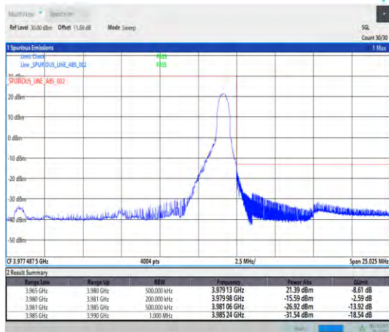
1-N77-3700-3980-PC2-30-15-H-2-DFT-QPSK-Edge_1 RB_Right-1@37-Ant1-1--PASS-see graph
