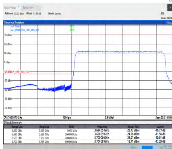
1-N77-3700-3980-PC2-30-15-L-3-DFT-QPSK-Outer_Full-36@0-Ant1-1--PASS-see graph
