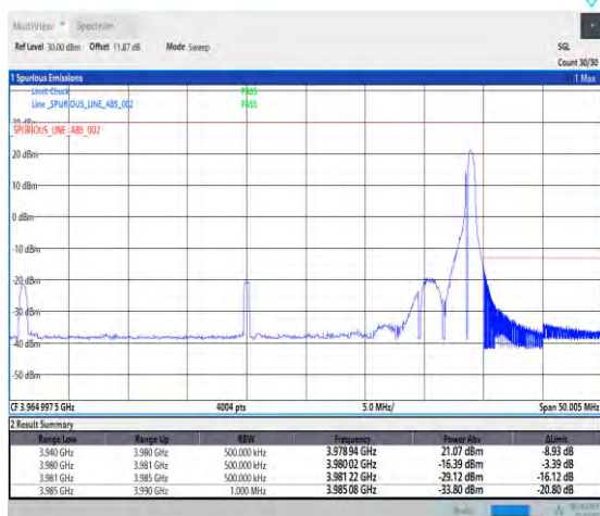
1-N77-3700-3980-PC2-30-40-H-2-DFT-QPSK-Edge_1 RB_Right-1@105-Ant1-1--PASS-see graph
