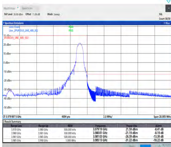
1-N77-3700-3980-PC2-30-10-H-5-CP-QPSK-Edge_1R B_Right-1@23-Ant1-1--PASS-see graph
