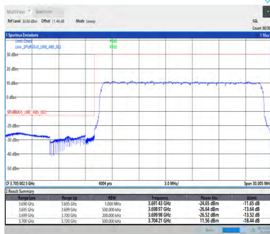
1-N77-3700-3980-PC2-30-20-L-3-DFT-QPSK-Outer_Full-50@0-Ant1-1--PASS-see graph
