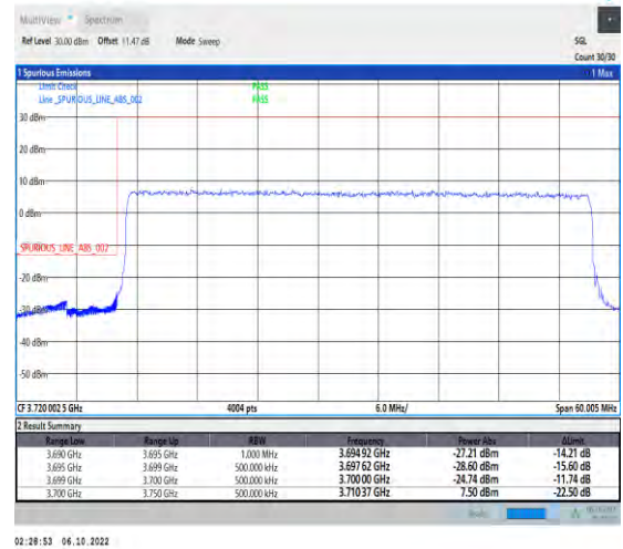
1-N77-3700-3980-PC2-30-50-L-3-DFT-QPSK-Outer_Full-128@0-Ant1-1--PASS-see graph
