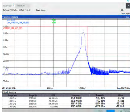
1-N77-3700-3980-PC2-30-20-H-2-DFT-QPSK-Edge_1 RB_Right-1@50-Ant1-1--PASS-see graph
