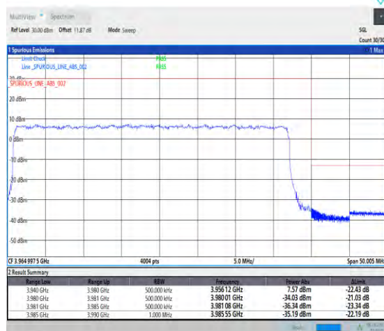
1-N77-3700-3980-PC2-30-40-H-3-DFT-QPSK-Out er_Full-100@0-Ant1-1--PASS-see graph
