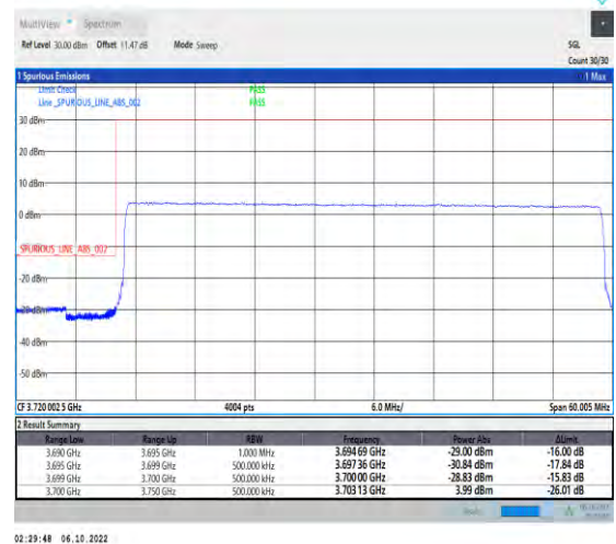
1-N77-3700-3980-PC2-30-50-L-6-CP-QPSK-Outer_Full-133@0-Ant1-1--PASS-see graph
