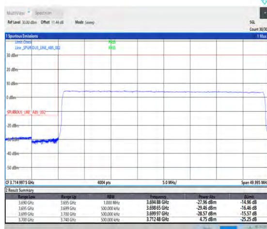
1-N77-3700-3980-PC2-30-40-L-6-CP-QPSK-Outer _Full-106@0-Ant1-1--PASS-see graph
