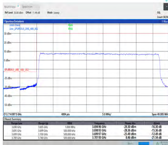
1-N77-3700-3980-PC2-30-40-L-3-DFT-QPSK-Outer _Full-100@0-Ant1-1--PASS-see graph
