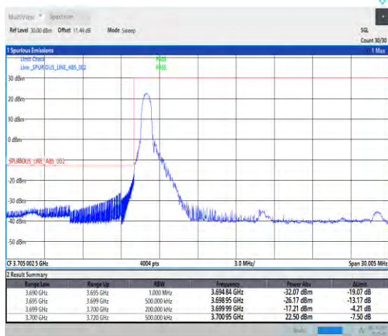
1-N77-3700-3980-PC2-30-20-L-1-DFT-QPSK-Edge_1 RB_Left-1@0-Ant1-1--PASS-see graph
