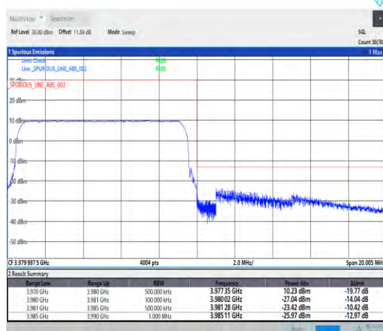
1-N77-3700-3980-PC2-30-10-H-6-CP-QPSK-Outer _Full-24@0-Ant1-1--PASS-see graph
