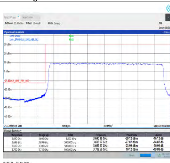
1-N77-3700-3980-PC2-30-30-L-3-DFT-QPSK-Outer_Full-75@0-Ant1-1--PASS-see graph
