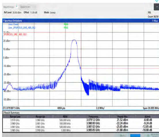
1-N77-3700-3980-PC2-30-10-H-2-DFT-QPSK-Edge_1 RB_Right-1@23-Ant1-1--PASS-see graph
