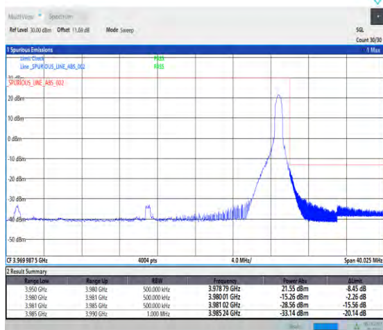
1-N77-3700-3980-PC2-30-30-H-2-DFT-QPSK-Edge_1 RB_Right-1@77-Ant1-1--PASS-see graph
