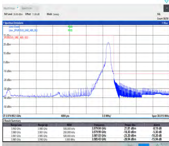
1-N77-3700-3980-PC2-30-20-H-5-CP-QPSK-Edge_1R B_Right-1@50-Ant1-1--PASS-see graph
