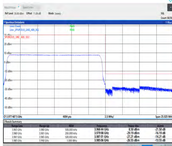
1-N77-3700-3980-PC2-30-15-H-6-CP-QPSK-Outer _Full-38@0-Ant1-1--PASS-see graph
