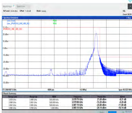
1-N77-3700-3980-PC2-30-30-H-5-CP-QPSK-Edge_1R B_Right-1@77-Ant1-1--PASS-see graph
