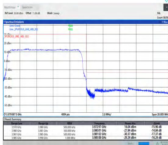
1-N77-3700-3980-PC2-30-10-H-3-DFT-QPSK-Out er_Full-24@0-Ant1-1--PASS-see graph
