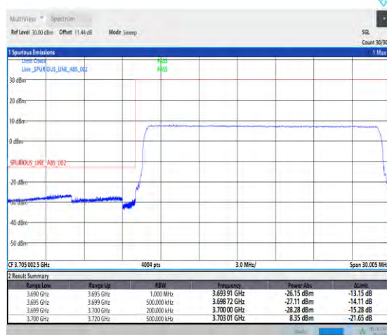
1-N77-3700-3980-PC2-30-20-L-6-CP-QPSK-Outer_Full-51@0-Ant1-1--PASS-see graph
