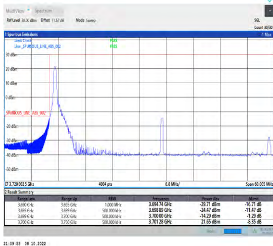
1-N77-3700-3980-PC2-30-50-L-4-CP-QPSK-Edge_1R B_Left-1@0-Ant1-1--PASS-see graph
