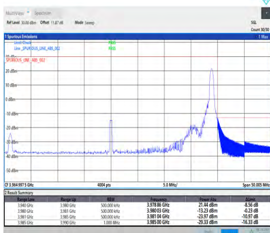
1-N77-3700-3980-PC2-30-40-H-5-CP-QPSK-Edge_1R B_Right-1@105-Ant1-1--PASS-see graph
