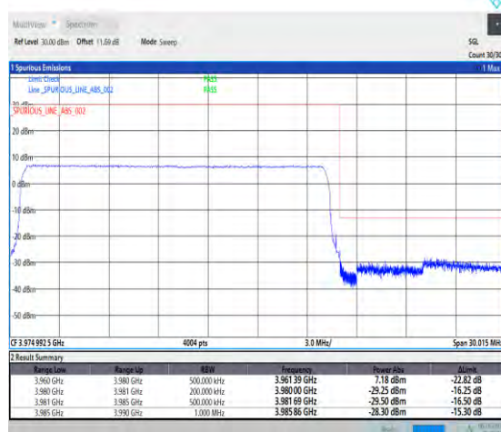
1-N77-3700-3980-PC2-30-20-H-6-CP-QPSK-Outer _Full-51@0-Ant1-1--PASS-see graph
