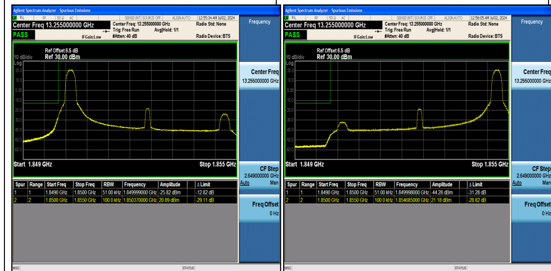
Band2_5MHz_QPSK_18625_1RB#0
