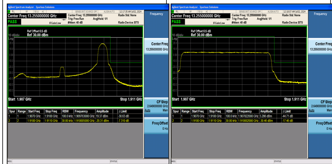
Band2_3MHz_64QAM_18615_15RB#0
