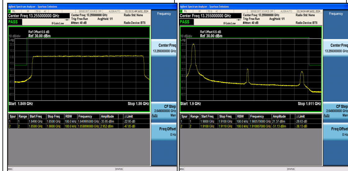
Band2_10MHz_QPSK_18650_50RB#0
