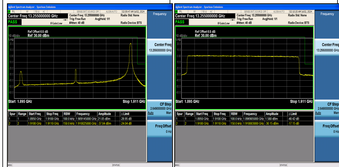
Band2_15MHz_QPSK_19125_1RB#74
