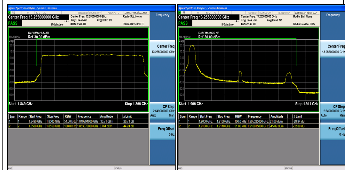
Band2_5MHz_QPSK_18625_1RB#0
