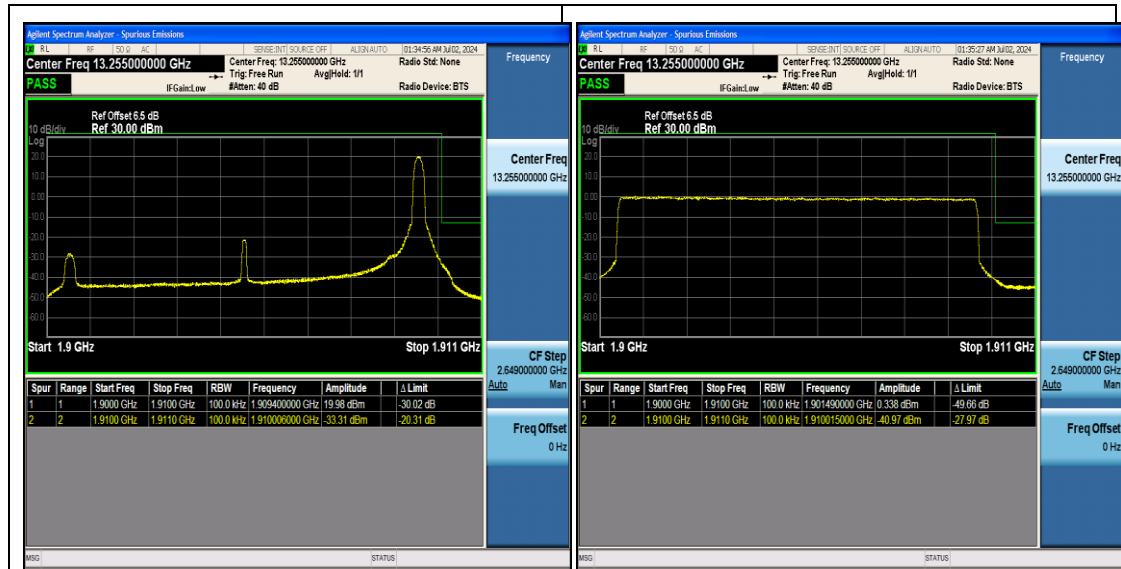
Band2_10MHz_64QAM_19150_1RB#49
