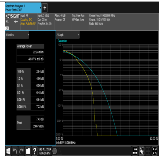
Band26(814-824)-10MHz-16QAM-26740-1RB#0-PASS
