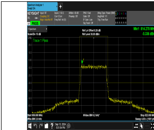
Band26_3MHz_QPSK_26705_15RB#0
