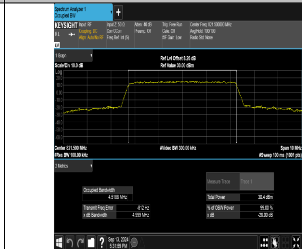
Band26(814-824)-5MHz-16QAM-26765-25RB#0-PASS
