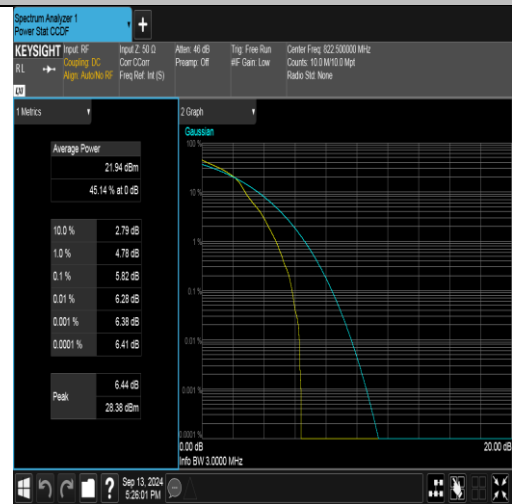
Band26(814-824)-3MHz-16QAM-26775-1RB#0-PASS
