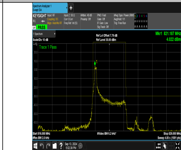
Band26_3MHz_16QAM_26775_1RB#0
