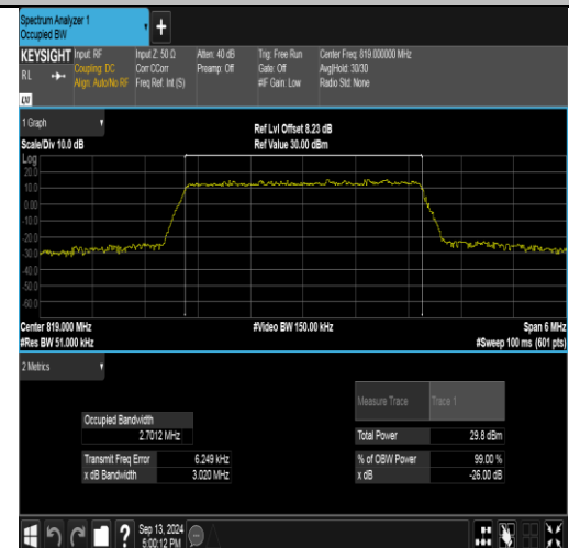
Band26(814-824)-3MHz-16QAM-26740-15RB#0-PASS
