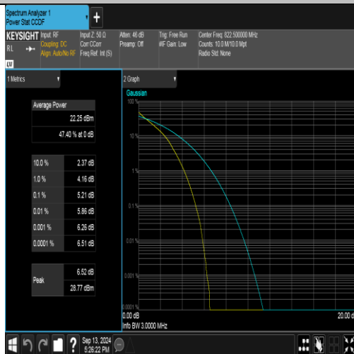
Band26(814-824)-3MHz-QPSK-26775-15RB#0-PASS
