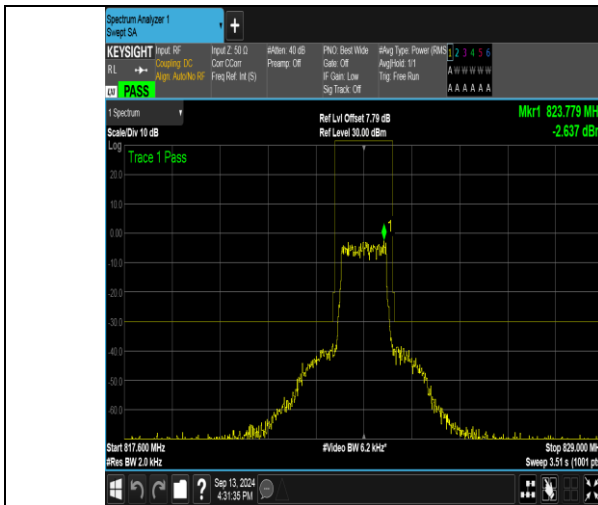
Band26_1.4MHz_QPSK_26783_6RB#0
