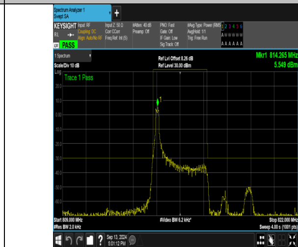
Band26_3MHz_16QAM_26705_1RB#0
