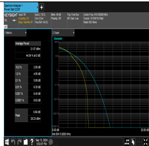
Band26(814-824)-5MHz-16QAM-26715-1RB#0-PASS
