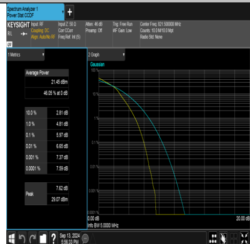
Band26(814-824)-5MHz-16QAM-26765-25RB#0-PASS
