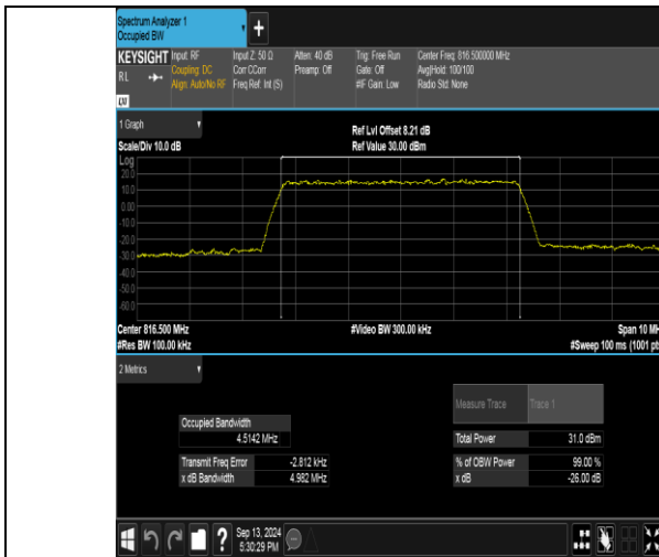
Band26(814-824)-5MHz-QPSK-26715-25RB#0-PASS
