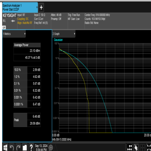
Band26(814-824)-5MHz-QPSK-26740-1RB#0-PASS
