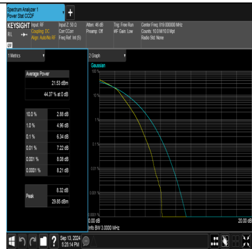
Band26(814-824)-3MHz-16QAM-26740-15RB#0-PASS
