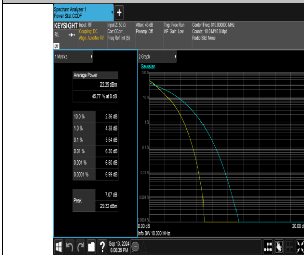
Band26(814-824)-10MHz-QPSK-26740-50RB#0-PASS
