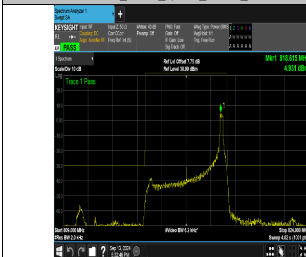
Band26_5MHz_QPSK_26715_1RB#24
