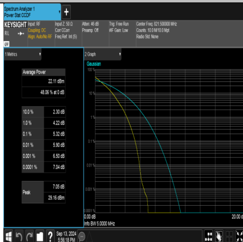
Band26(814-824)-5MHz-QPSK-26765-25RB#0-PASS
