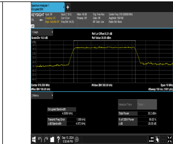
Band26(814-824)-5MHz-16QAM-26715-25RB#0-PASS
