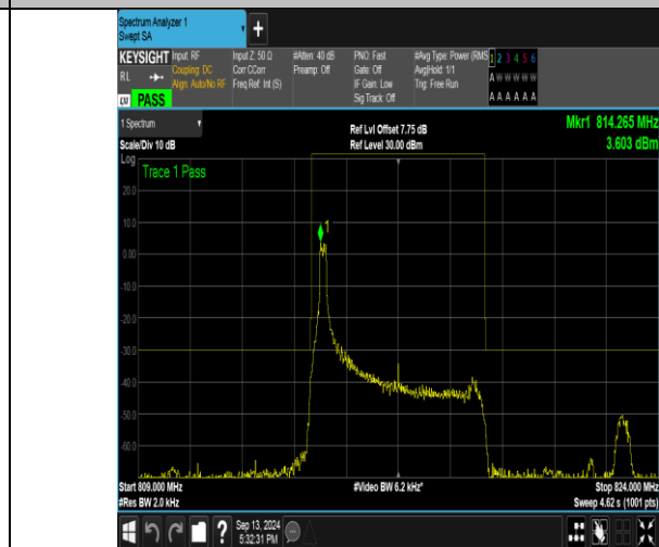
Band26_5MHz_16QAM_26715_1RB#0
