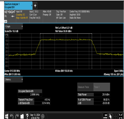
Band26(814-824)-3MHz-16QAM-26705-15RB#0-PASS
