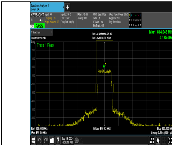
Band26_1.4MHz_QPSK_26697_6RB#0
