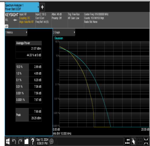
Band26(814-824)-10MHz-16QAM-26740-50RB#0-PASS
