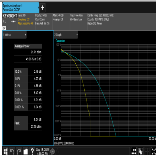
Band26(814-824)-1.4MHz-QPSK-26783-6RB#0-PASS
