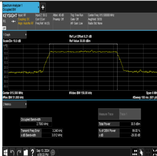
Band26(814-824)-3MHz-QPSK-26705-15RB#0-PASS
