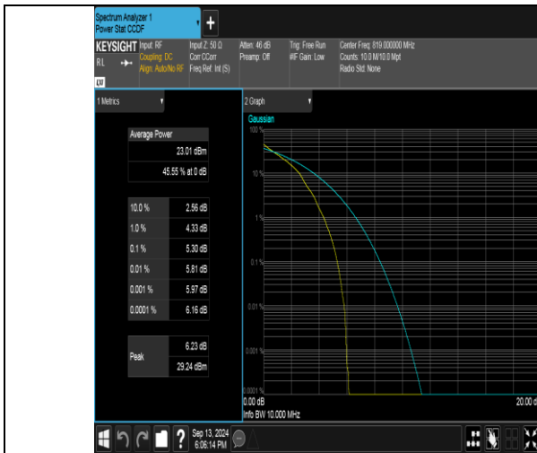
Band26(814-824)-10MHz-QPSK-26740-1RB#0-PASS
