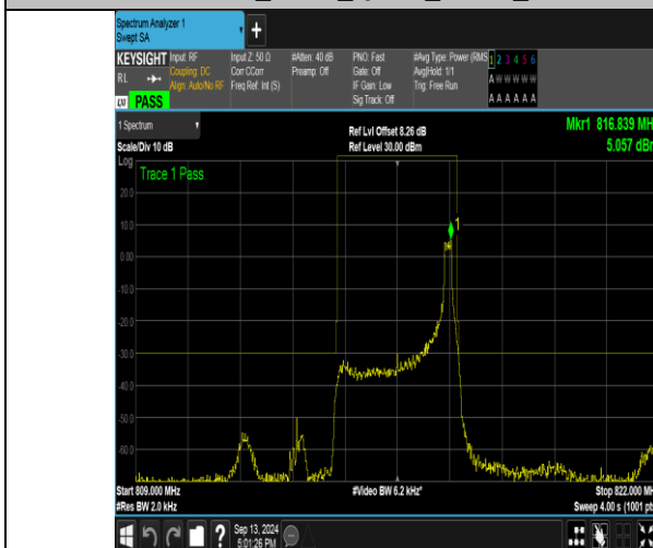
Band26_3MHz_QPSK_26705_1RB#14
