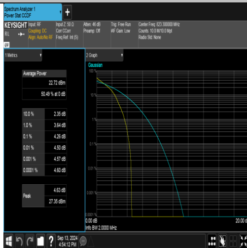
Band26(814-824)-1.4MHz-QPSK-26783-1RB#0-PASS
