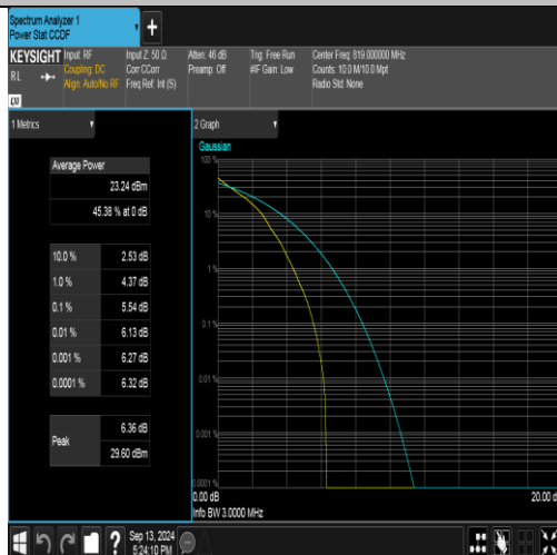
Band26(814-824)-3MHz-QPSK-26740-1RB#0-PASS
