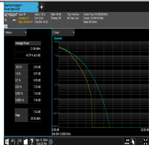
Band26(814-824)-3MHz-16QAM-26740-1RB#0-PASS
