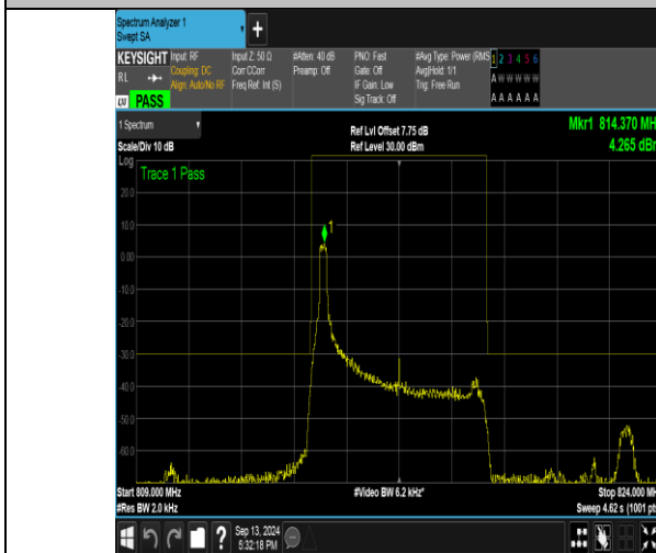
Band26_5MHz_QPSK_26715_1RB#0
