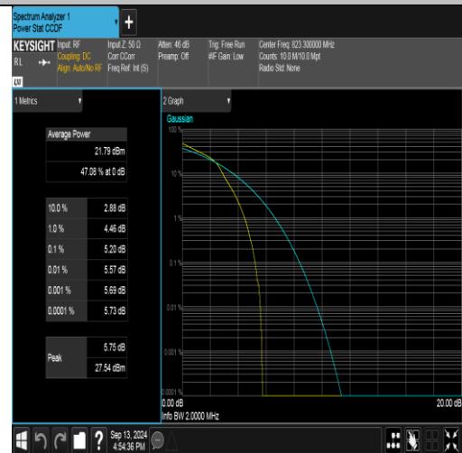
Band26(814-824)-1.4MHz-16QAM-26783-1RB#0-PASS
