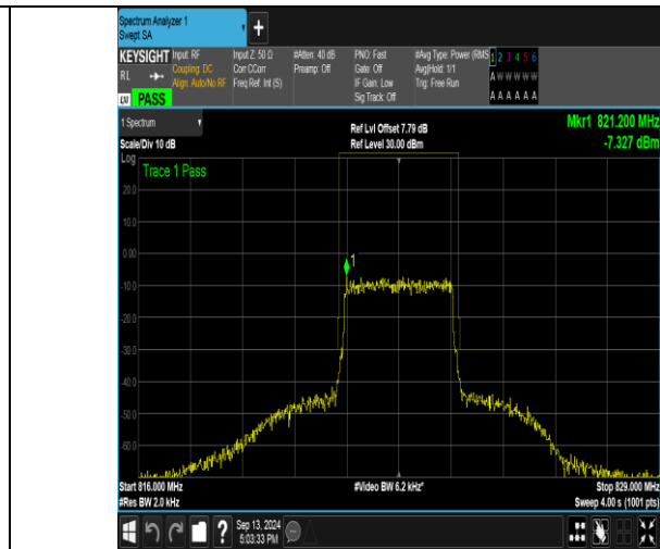
Band26_3MHz_16QAM_26775_15RB#0
