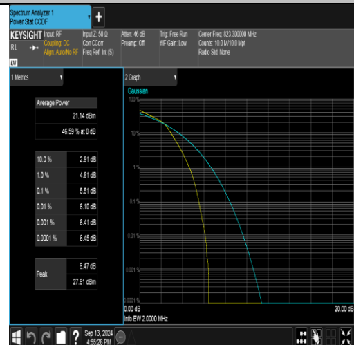
Band26(814-824)-1.4MHz-16QAM-26783-6RB#0-PASS
