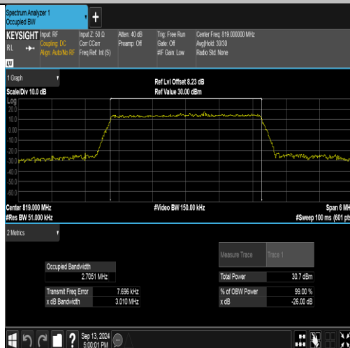
Band26(814-824)-3MHz-QPSK-26740-15RB#0-PASS
