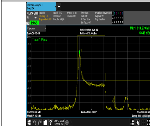
Band26_3MHz_QPSK_26705_1RB#0
