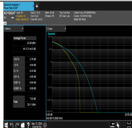
Band26(814-824)-5MHz-16QAM-26740-1RB#0-PASS
