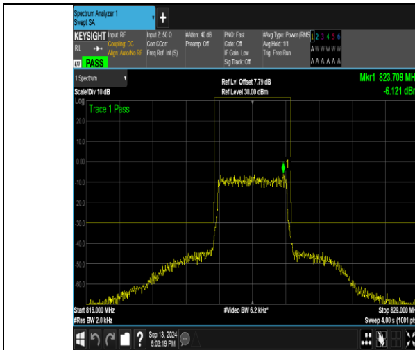
Band26_3MHz_QPSK_26775_15RB#0
