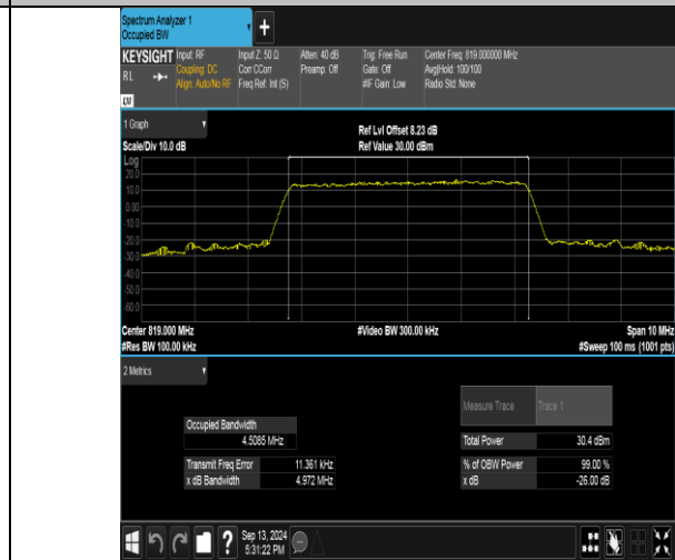
Band26(814-824)-5MHz-16QAM-26740-25RB#0-PASS
