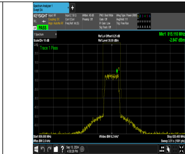
Band26_1.4MHz_16QAM_26697_6RB#0
