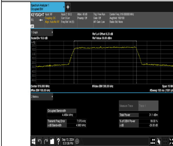
Band26(814-824)-5MHz-QPSK-26740-25RB#0-PASS
