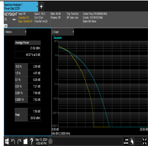
Band26(814-824)-1.4MHz-16QAM-26740-6RB#0-PASS
