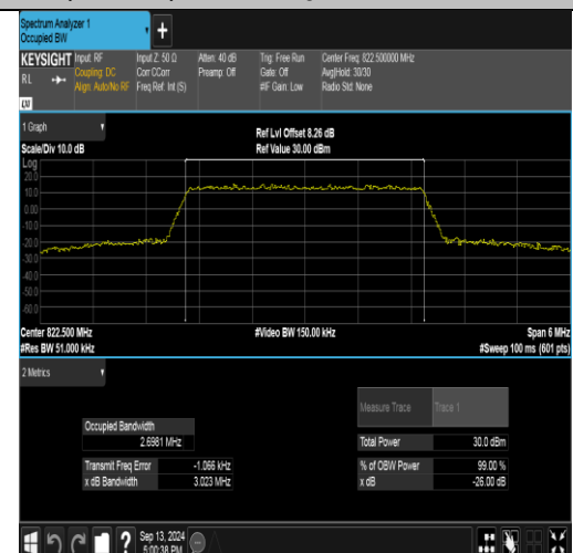
Band26(814-824)-3MHz-16QAM-26775-15RB#0-PASS
