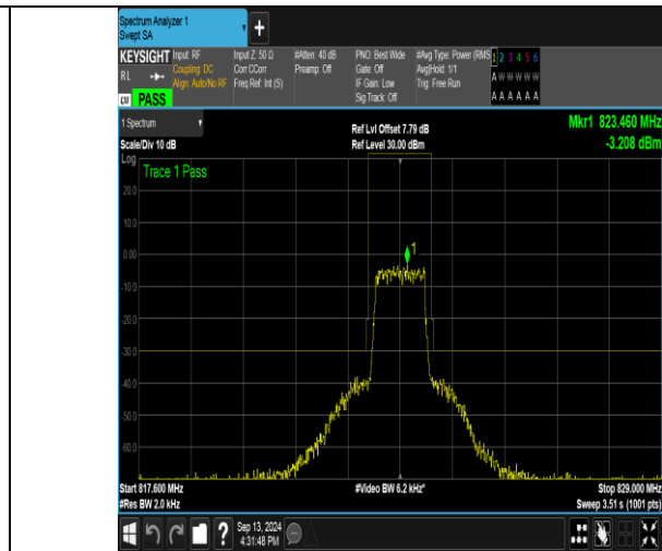
Band26_1.4MHz_16QAM_26783_6RB#0
