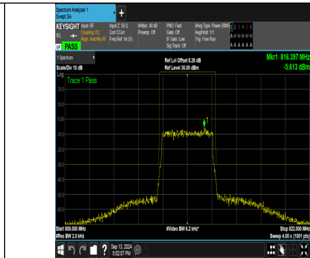
Band26_3MHz_16QAM_26705_15RB#0
