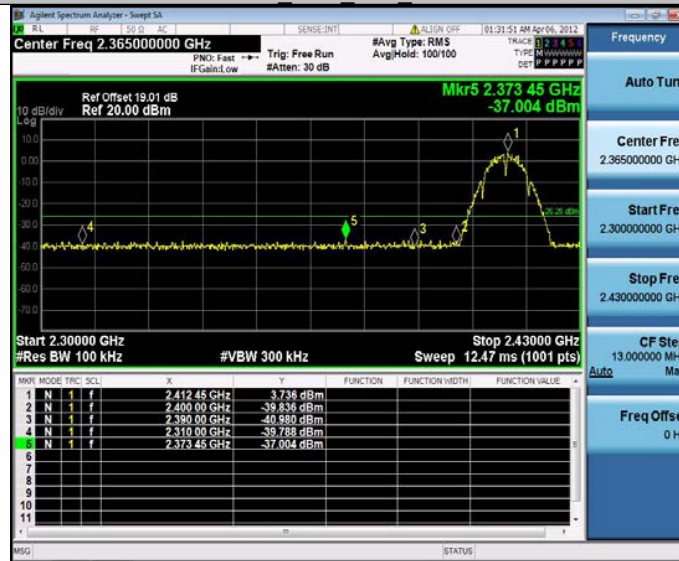
11B_Ant2_Low_2412
