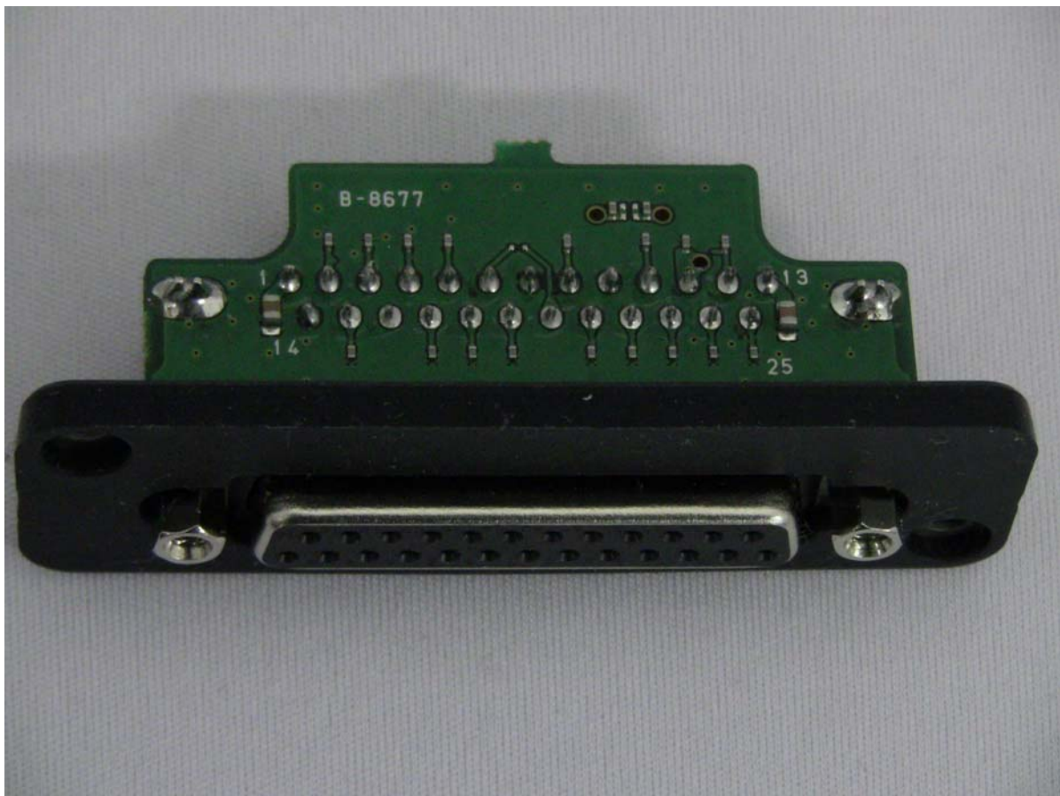
IC-F7520 CONNECT-B UNIT B SIDE
