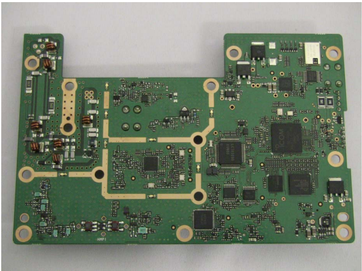
IC-F7520 MAIN-B UNIT B SIDE
