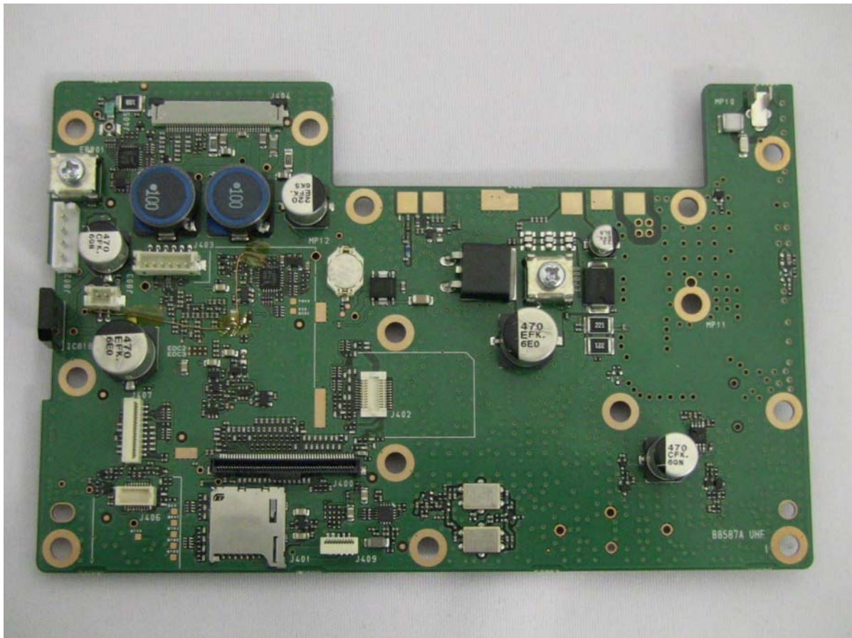
IC-F7520 MAIN-B UNIT A SIDE
