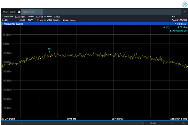
GFSK on Channel 39
