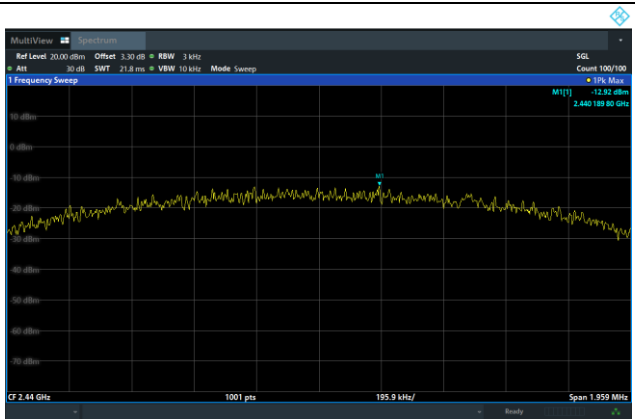
GFSK on Channel 19
