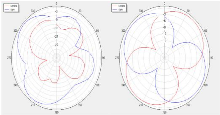
H Theta=90 freq=1740MHz
