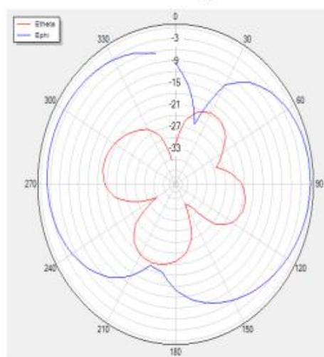
H Theta=90 freq=780MHz
