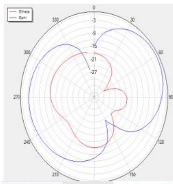
H Theta=90 freq=960MHz
