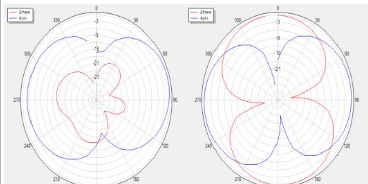
H Theta=90 freq=840MHz
