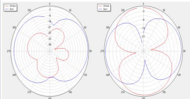
H Theta=90 freq=840MHz
