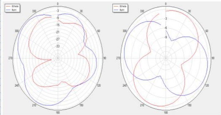
H Theta=90 freq=1780MHz
