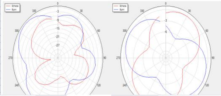
H Theta=90 freq=1780MHz
