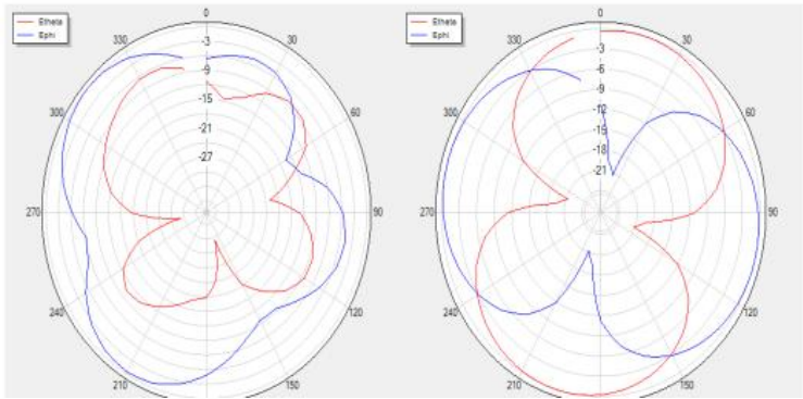
H Theta=90 freq=1740MHz
