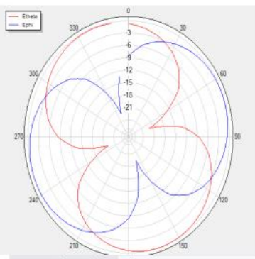
H Theta=0 freq=960MHz
