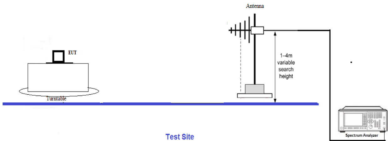
Block Diagram Rev. C
