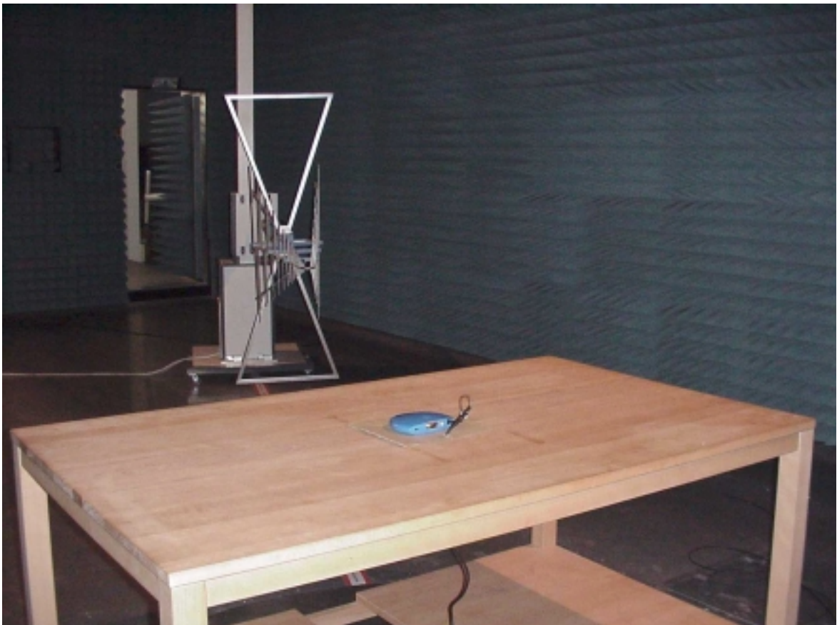
radiated measurements - test setup
