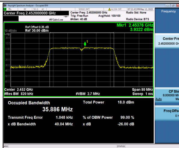
11N40SISO_Ant1_2452
