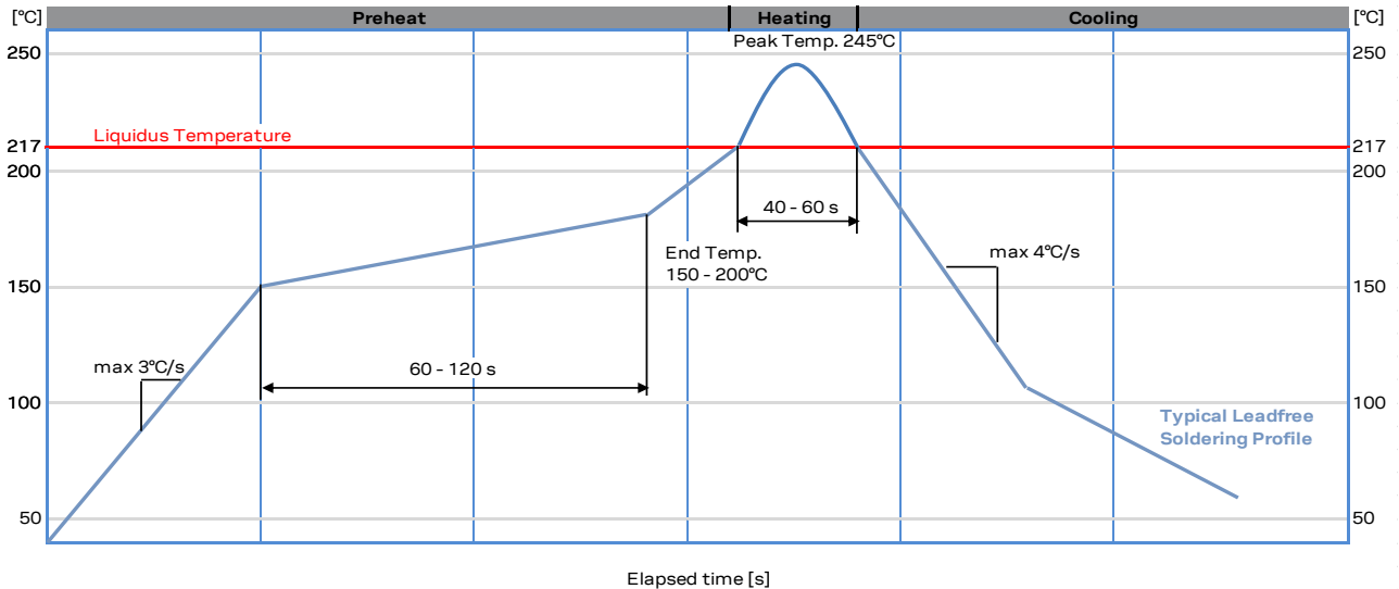
Figure 67: Recommended soldering profile
