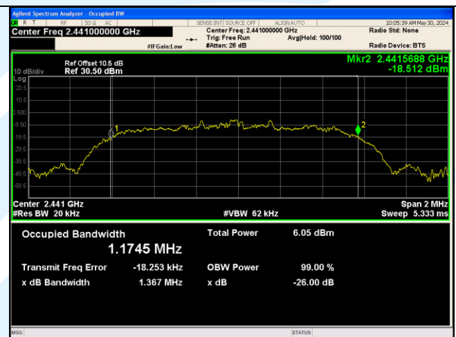
8DPSK_3-DH5_Channel 39
